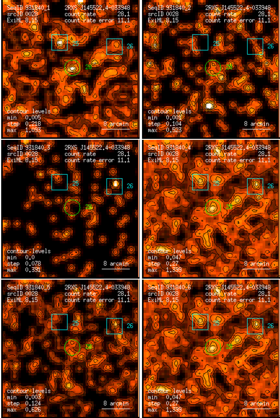
Figure 28: RASS 931840: detection 0028: band rate images, Gaussian filter: (1) PSPC channels 11 – 41, (2) 52 – 90, (3) 91 – 201, (4) 11 – 235, (5) 52 – 201, (6) 11 – 201. Broad band rates in counts/ks. Band rate contour levels in counts/ks/arcmin 2 .
