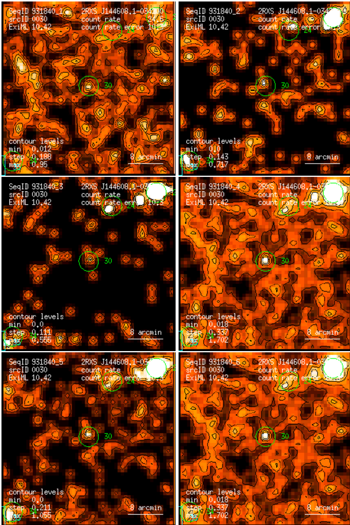
Figure 30: RASS 931840: detection 0030: band rate images, Gaussian filter: (1) PSPC channels 11 – 41, (2) 52 – 90, (3) 91 – 201, (4) 11 – 235, (5) 52 – 201, (6) 11 – 201. Broad band rates in counts/ks. Band rate contour levels in counts/ks/arcmin 2 .
