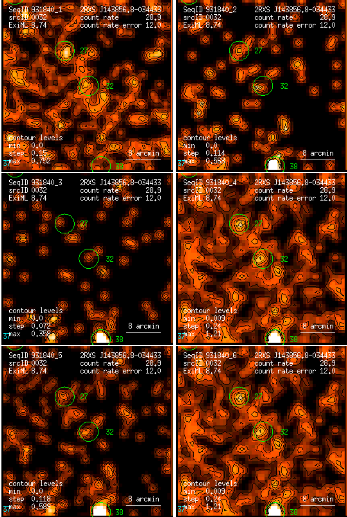
Figure 32: RASS 931840: detection 0032: band rate images, Gaussian filter: (1) PSPC channels 11 – 41, (2) 52 – 90, (3) 91 – 201, (4) 11 – 235, (5) 52 – 201, (6) 11 – 201. Broad band rates in counts/ks. Band rate contour levels in counts/ks/arcmin 2 .
