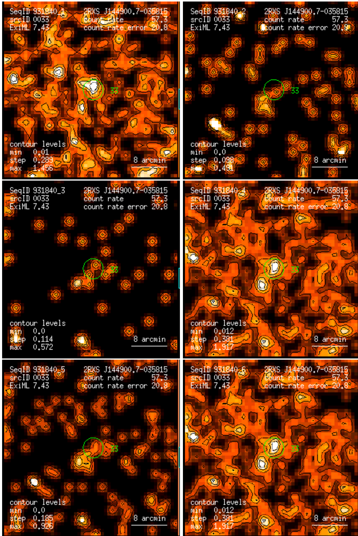
Figure 33: RASS 931840: detection 0033: band rate images, Gaussian filter: (1) PSPC channels 11 – 41, (2) 52 – 90, (3) 91 – 201, (4) 11 – 235, (5) 52 – 201, (6) 11 – 201. Broad band rates in counts/ks. Band rate contour levels in counts/ks/arcmin 2 .
