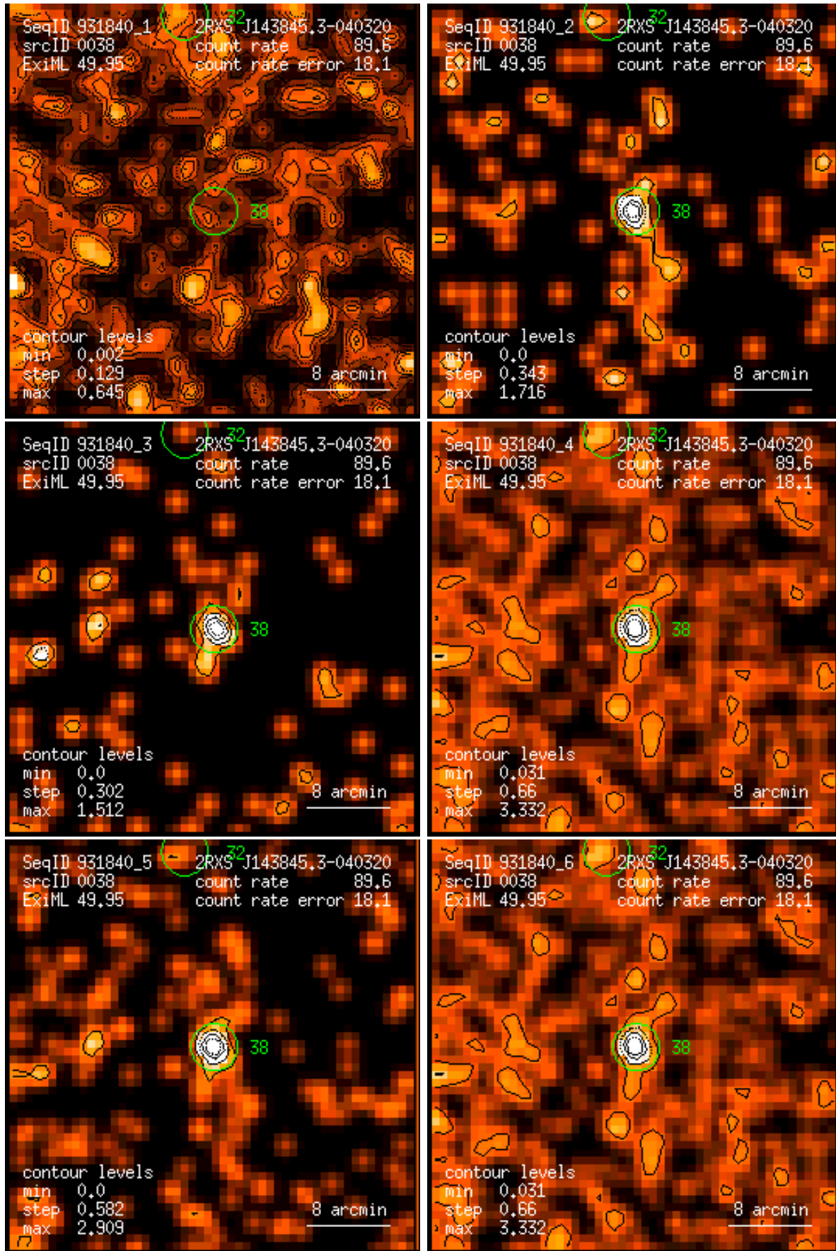
Figure 38: RASS 931840: detection 0038: band rate images, Gaussian filter: (1) PSPC channels 11 – 41, (2) 52 – 90, (3) 91 – 201, (4) 11 – 235, (5) 52 – 201, (6) 11 – 201. Broad band rates in counts/ks. Band rate contour levels in counts/ks/arcmin 2 .
