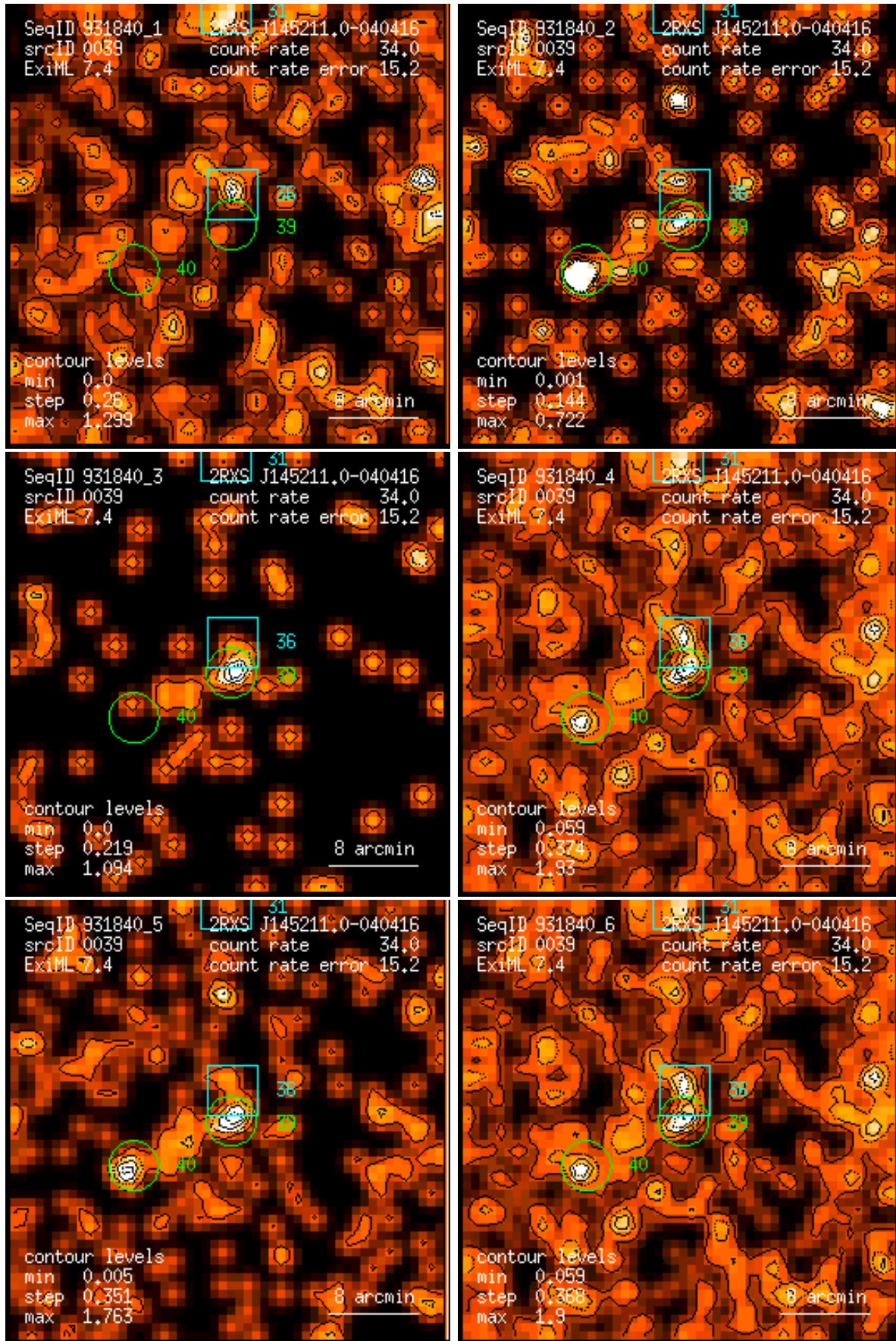
Figure 39: RASS 931840: detection 0039: band rate images, Gaussian filter: (1) PSPC channels 11 – 41, (2) 52 – 90, (3) 91 – 201, (4) 11 – 235, (5) 52 – 201, (6) 11 – 201. Broad band rates in counts/ks. Band rate contour levels in counts/ks/arcmin 2 .
