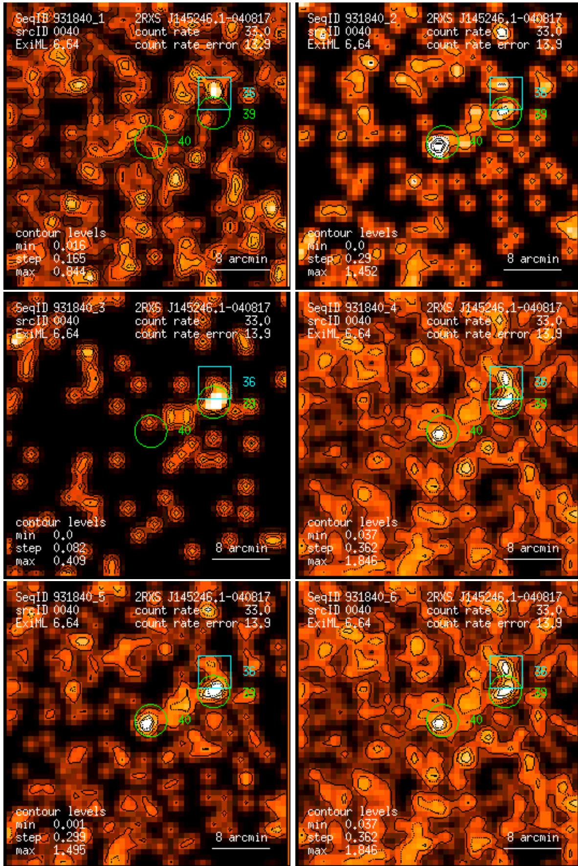
Figure 40: RASS 931840: detection 0040: band rate images, Gaussian filter: (1) PSPC channels 11 – 41, (2) 52 – 90, (3) 91 – 201, (4) 11 – 235, (5) 52 – 201, (6) 11 – 201. Broad band rates in counts/ks. Band rate contour levels in counts/ks/arcmin 2 .
