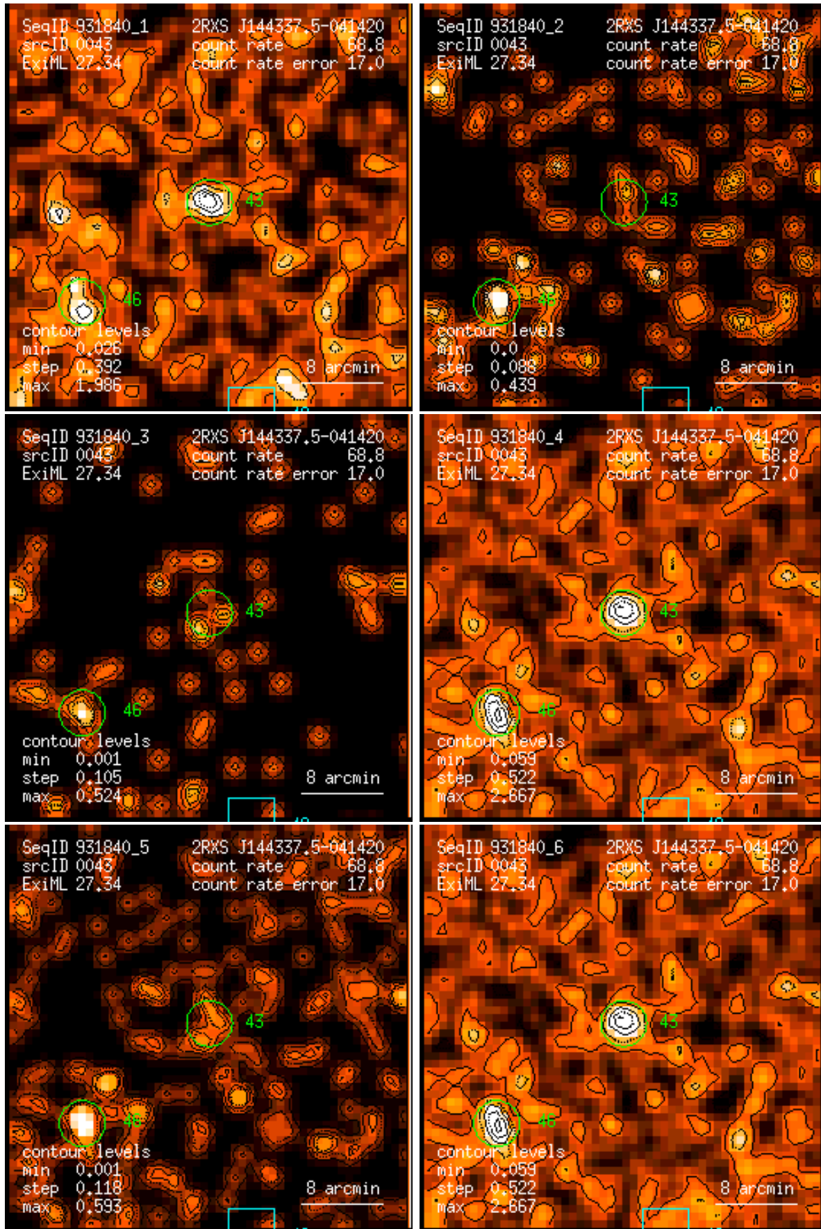
Figure 43: RASS 931840: detection 0043: band rate images, Gaussian filter: (1) PSPC channels 11 – 41, (2) 52 – 90, (3) 91 – 201, (4) 11 – 235, (5) 52 – 201, (6) 11 – 201. Broad band rates in counts/ks. Band rate contour levels in counts/ks/arcmin 2 .
