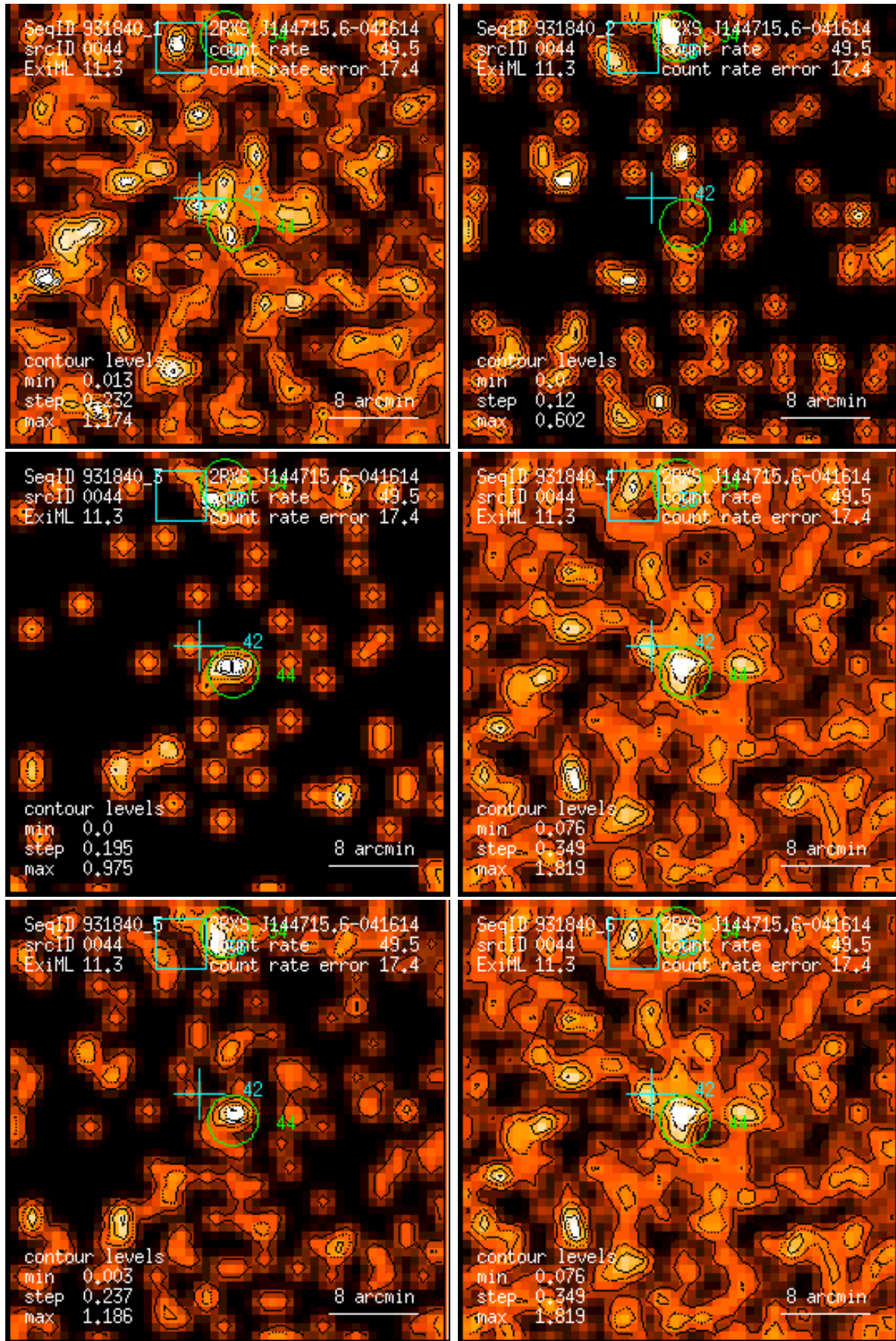
Figure 44: RASS 931840: detection 0044: band rate images, Gaussian filter: (1) PSPC channels 11 – 41, (2) 52 – 90, (3) 91 – 201, (4) 11 – 235, (5) 52 – 201, (6) 11 – 201. Broad band rates in counts/ks. Band rate contour levels in counts/ks/arcmin 2 .
