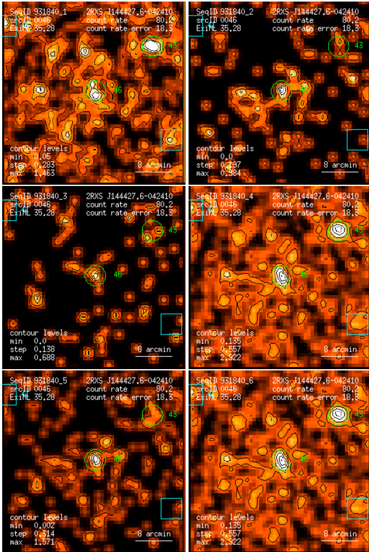
Figure 46: RASS 931840: detection 0046: band rate images, Gaussian filter: (1) PSPC channels 11 – 41, (2) 52 – 90, (3) 91 – 201, (4) 11 – 235, (5) 52 – 201, (6) 11 – 201. Broad band rates in counts/ks. Band rate contour levels in counts/ks/arcmin 2 .
