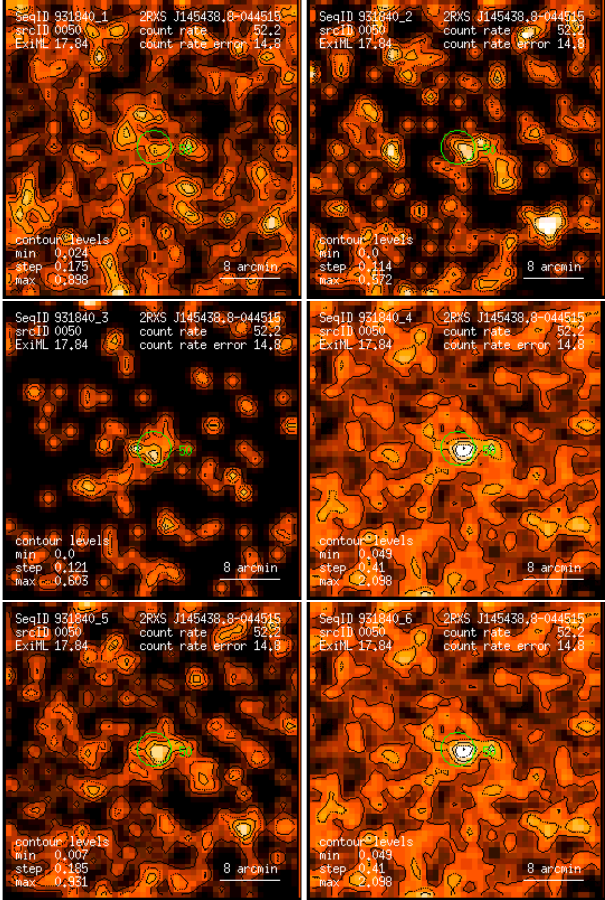
Figure 50: RASS 931840: detection 0050: band rate images, Gaussian filter: (1) PSPC channels 11 – 41, (2) 52 – 90, (3) 91 – 201, (4) 11 – 235, (5) 52 – 201, (6) 11 – 201. Broad band rates in counts/ks. Band rate contour levels in counts/ks/arcmin 2 .
