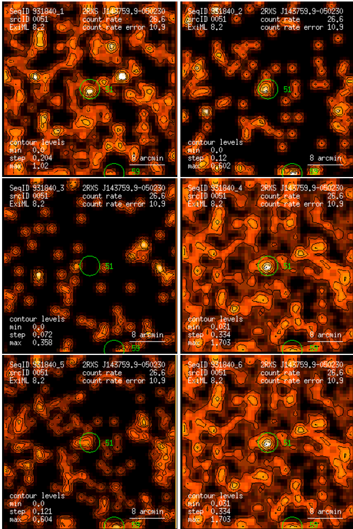
Figure 51: RASS 931840: detection 0051: band rate images, Gaussian filter: (1) PSPC channels 11 – 41, (2) 52 – 90, (3) 91 – 201, (4) 11 – 235, (5) 52 – 201, (6) 11 – 201. Broad band rates in counts/ks. Band rate contour levels in counts/ks/arcmin 2 .
