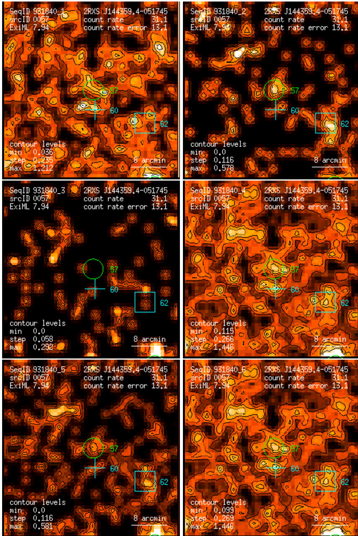
Figure 57: RASS 931840: detection 0057: band rate images, Gaussian filter: (1) PSPC channels 11 – 41, (2) 52 – 90, (3) 91 – 201, (4) 11 – 235, (5) 52 – 201, (6) 11 – 201. Broad band rates in counts/ks. Band rate contour levels in counts/ks/arcmin 2 .
