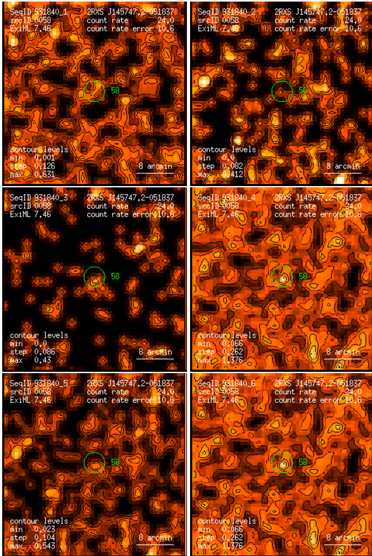
Figure 58: RASS 931840: detection 0058: band rate images, Gaussian filter: (1) PSPC channels 11 – 41, (2) 52 – 90, (3) 91 – 201, (4) 11 – 235, (5) 52 – 201, (6) 11 – 201. Broad band rates in counts/ks. Band rate contour levels in counts/ks/arcmin 2 .
