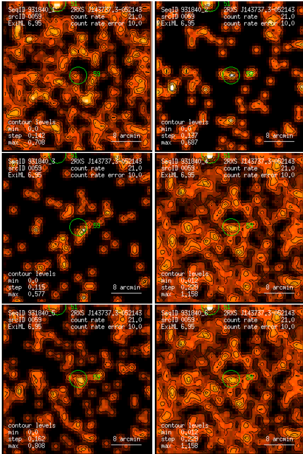
Figure 59: RASS 931840: detection 0059: band rate images, Gaussian filter: (1) PSPC channels 11 – 41, (2) 52 – 90, (3) 91 – 201, (4) 11 – 235, (5) 52 – 201, (6) 11 – 201. Broad band rates in counts/ks. Band rate contour levels in counts/ks/arcmin 2 .
