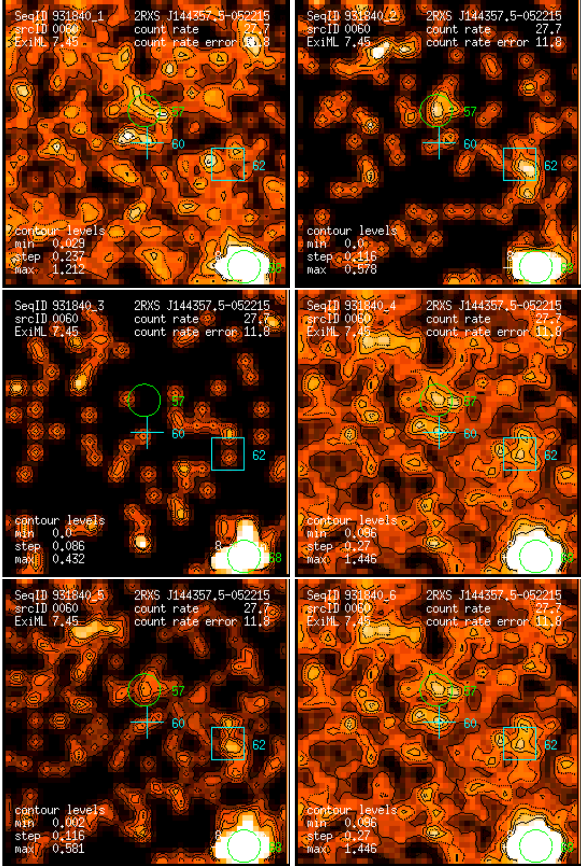
Figure 60: RASS 931840: detection 0060: band rate images, Gaussian filter: (1) PSPC channels 11 – 41, (2) 52 – 90, (3) 91 – 201, (4) 11 – 235, (5) 52 – 201, (6) 11 – 201. Broad band rates in counts/ks. Band rate contour levels in counts/ks/arcmin 2 .
