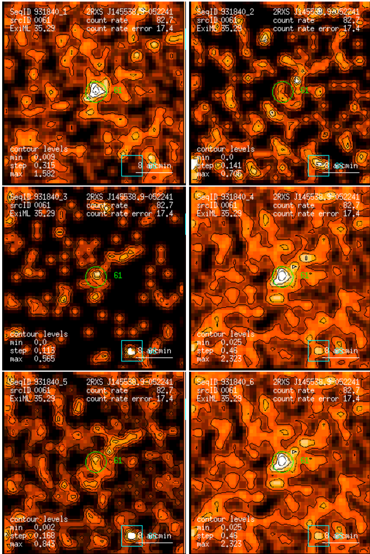
Figure 61: RASS 931840: detection 0061: band rate images, Gaussian filter: (1) PSPC channels 11 – 41, (2) 52 – 90, (3) 91 – 201, (4) 11 – 235, (5) 52 – 201, (6) 11 – 201. Broad band rates in counts/ks. Band rate contour levels in counts/ks/arcmin 2 .
