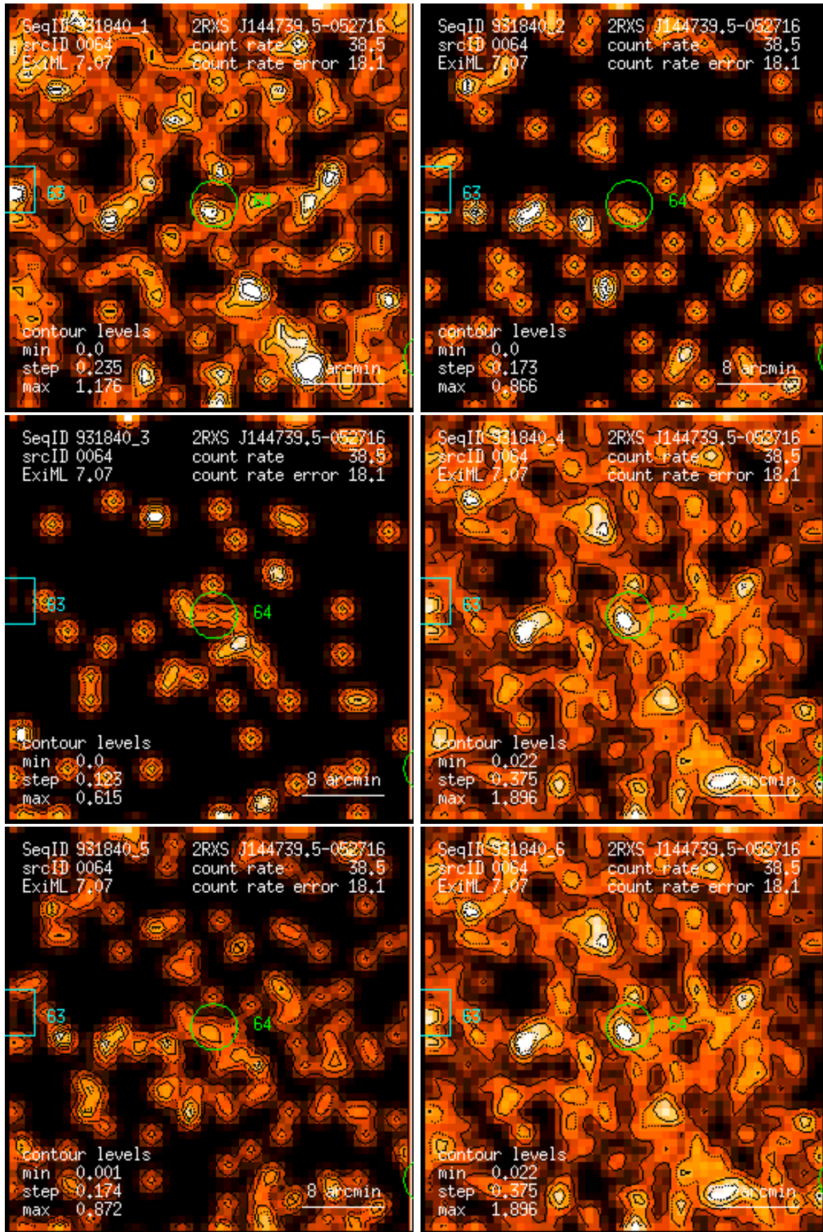
Figure 64: RASS 931840: detection 0064: band rate images, Gaussian filter: (1) PSPC channels 11 – 41, (2) 52 – 90, (3) 91 – 201, (4) 11 – 235, (5) 52 – 201, (6) 11 – 201. Broad band rates in counts/ks. Band rate contour levels in counts/ks/arcmin 2 .
