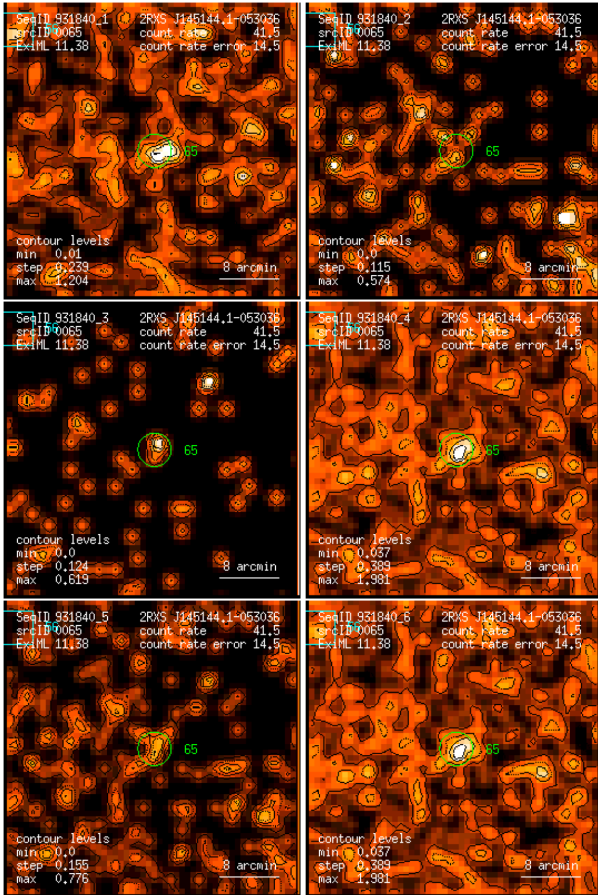
Figure 65: RASS 931840: detection 0065: band rate images, Gaussian filter: (1) PSPC channels 11 – 41, (2) 52 – 90, (3) 91 – 201, (4) 11 – 235, (5) 52 – 201, (6) 11 – 201. Broad band rates in counts/ks. Band rate contour levels in counts/ks/arcmin 2 .
