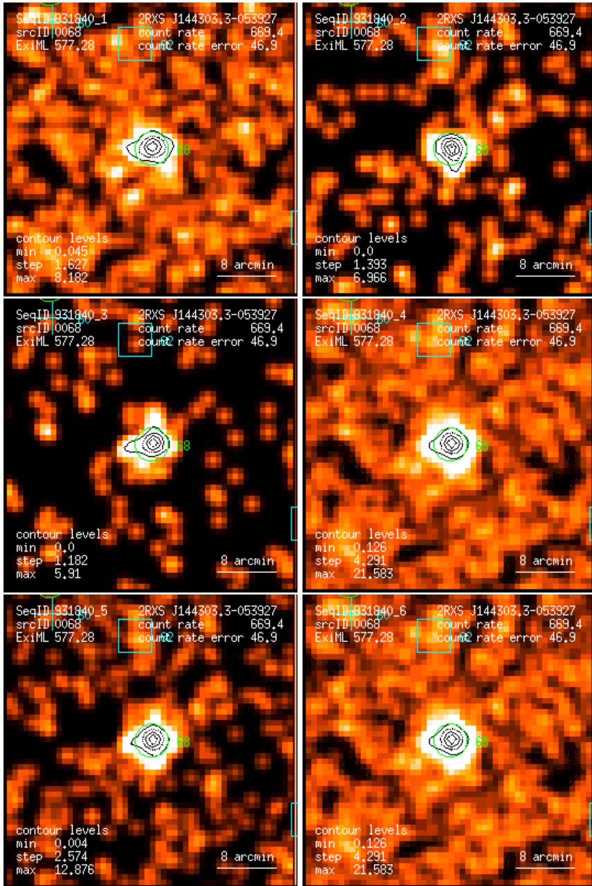
Figure 68: RASS 931840: detection 0068: band rate images, Gaussian filter: (1) PSPC channels 11 – 41, (2) 52 – 90, (3) 91 – 201, (4) 11 – 235, (5) 52 – 201, (6) 11 – 201. Broad band rates in counts/ks. Band rate contour levels in counts/ks/arcmin 2 .
