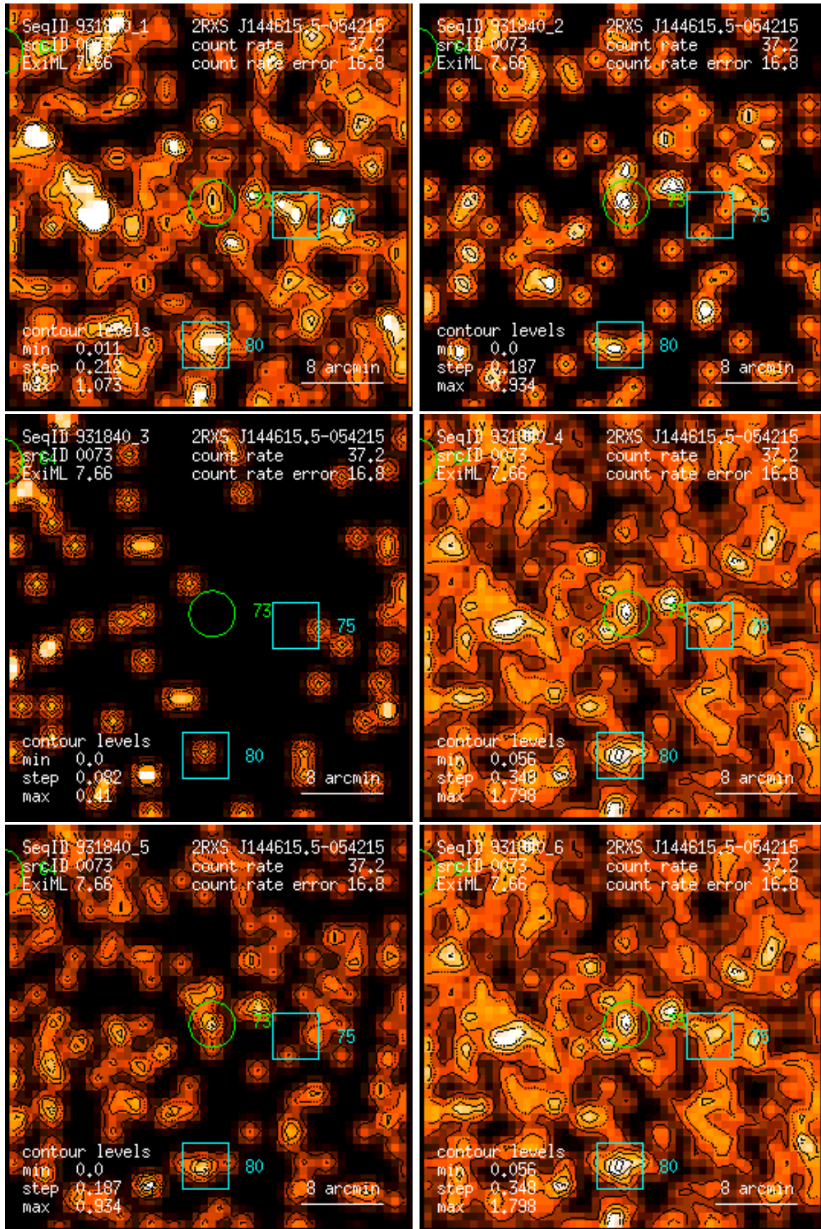
Figure 73: RASS 931840: detection 0073: band rate images, Gaussian filter: (1) PSPC channels 11 – 41, (2) 52 – 90, (3) 91 – 201, (4) 11 – 235, (5) 52 – 201, (6) 11 – 201. Broad band rates in counts/ks. Band rate contour levels in counts/ks/arcmin 2 .
