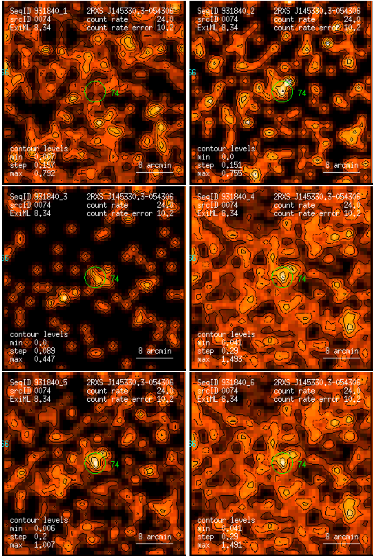
Figure 74: RASS 931840: detection 0074: band rate images, Gaussian filter: (1) PSPC channels 11 – 41, (2) 52 – 90, (3) 91 – 201, (4) 11 – 235, (5) 52 – 201, (6) 11 – 201. Broad band rates in counts/ks. Band rate contour levels in counts/ks/arcmin 2 .
