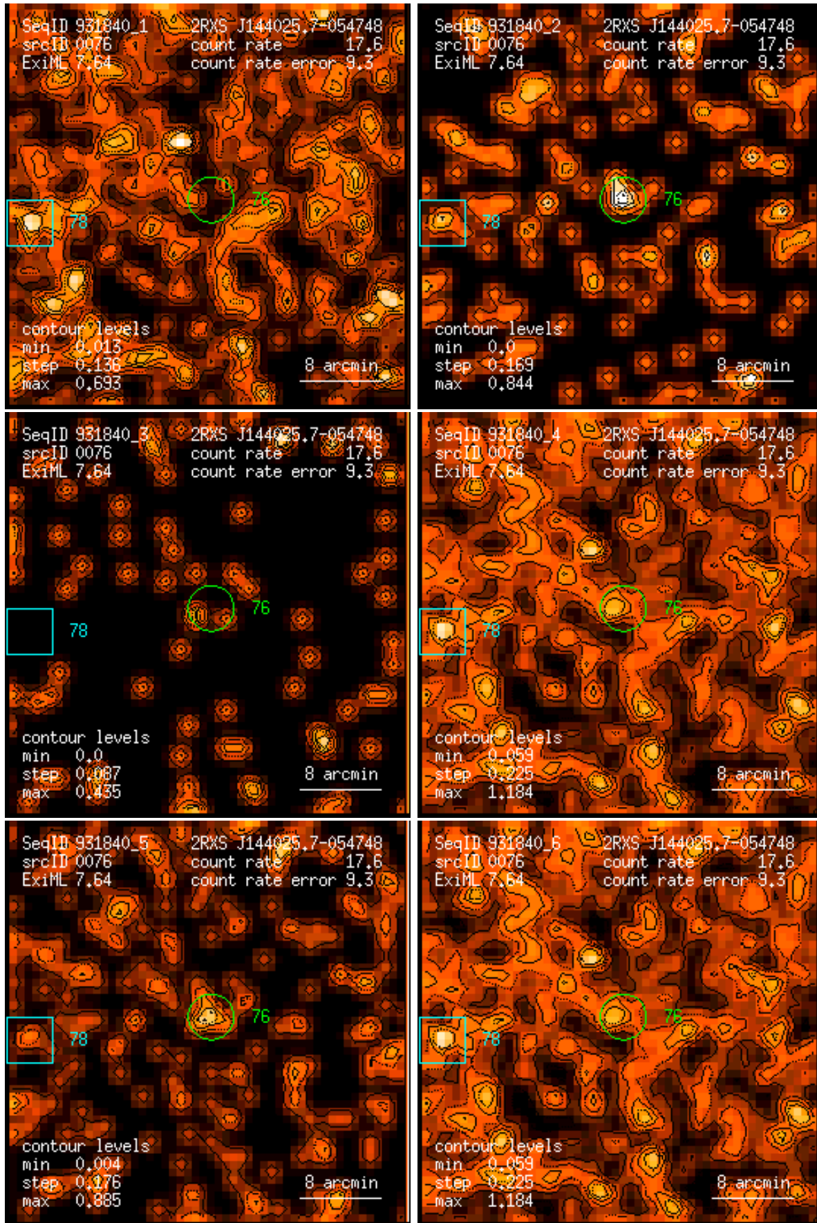
Figure 76: RASS 931840: detection 0076: band rate images, Gaussian filter: (1) PSPC channels 11 – 41, (2) 52 – 90, (3) 91 – 201, (4) 11 – 235, (5) 52 – 201, (6) 11 – 201. Broad band rates in counts/ks. Band rate contour levels in counts/ks/arcmin 2 .
