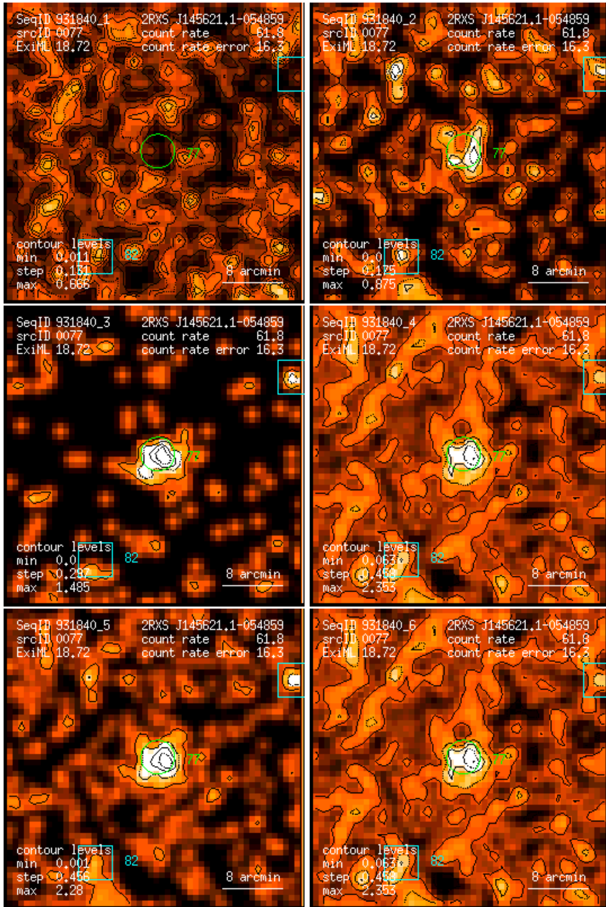
Figure 77: RASS 931840: detection 0077: band rate images, Gaussian filter: (1) PSPC channels 11 – 41, (2) 52 – 90, (3) 91 – 201, (4) 11 – 235, (5) 52 – 201, (6) 11 – 201. Broad band rates in counts/ks. Band rate contour levels in counts/ks/arcmin 2 .
