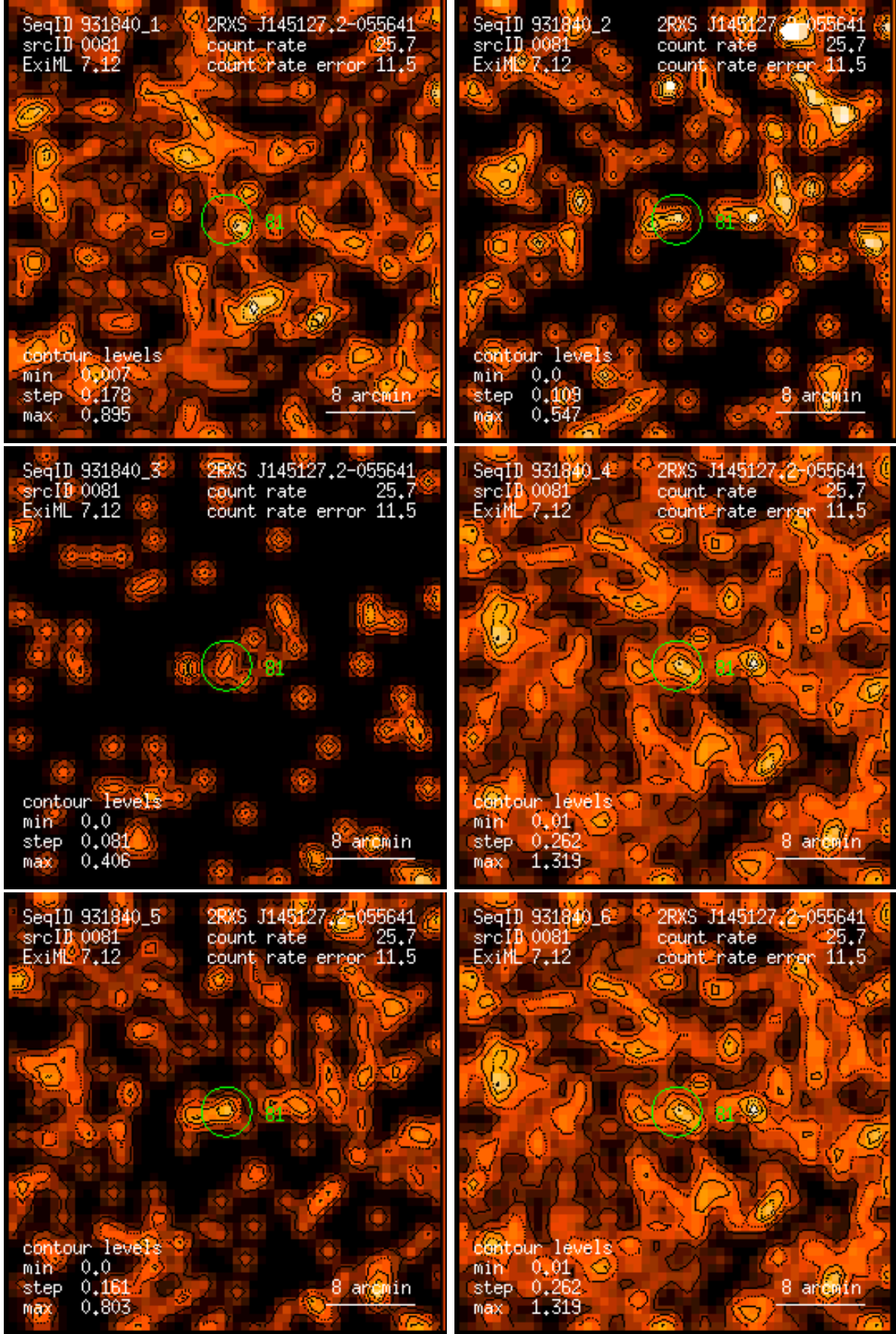
Figure 81: RASS 931840: detection 0081: band rate images, Gaussian filter: (1) PSPC channels 11 – 41, (2) 52 – 90, (3) 91 – 201, (4) 11 – 235, (5) 52 – 201, (6) 11 – 201. Broad band rates in counts/ks. Band rate contour levels in counts/ks/arcmin 2 .
