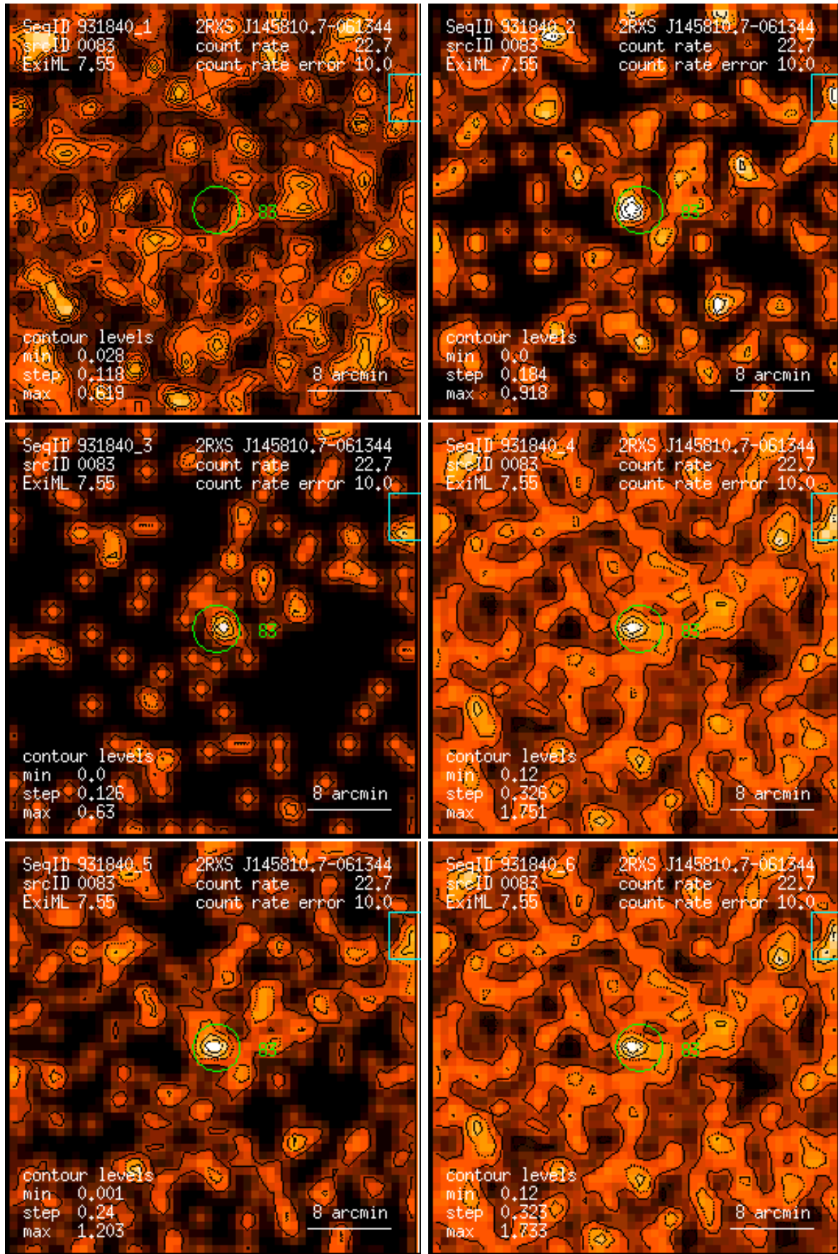
Figure 83: RASS 931840: detection 0083: band rate images, Gaussian filter: (1) PSPC channels 11 – 41, (2) 52 – 90, (3) 91 – 201, (4) 11 – 235, (5) 52 – 201, (6) 11 – 201. Broad band rates in counts/ks. Band rate contour levels in counts/ks/arcmin 2 .
