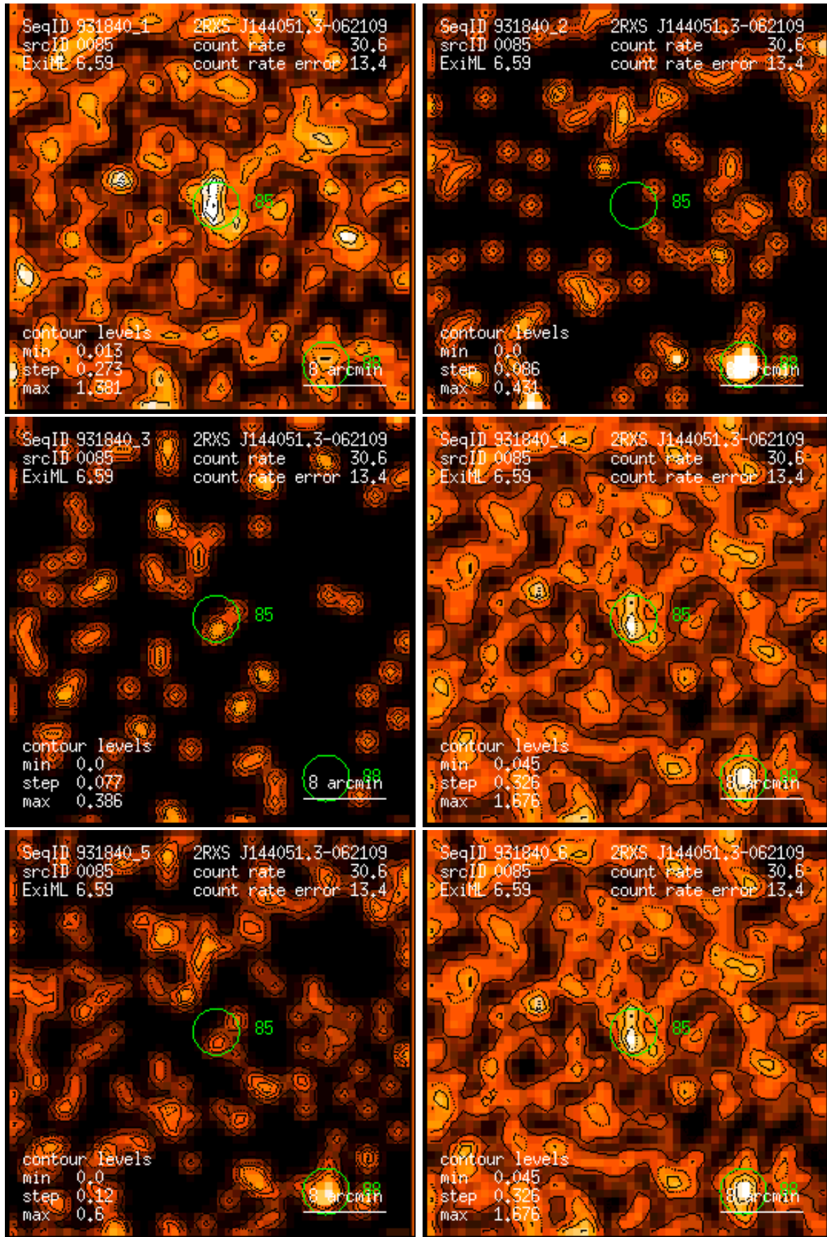
Figure 85: RASS 931840: detection 0085: band rate images, Gaussian filter: (1) PSPC channels 11 – 41, (2) 52 – 90, (3) 91 – 201, (4) 11 – 235, (5) 52 – 201, (6) 11 – 201. Broad band rates in counts/ks. Band rate contour levels in counts/ks/arcmin 2 .
