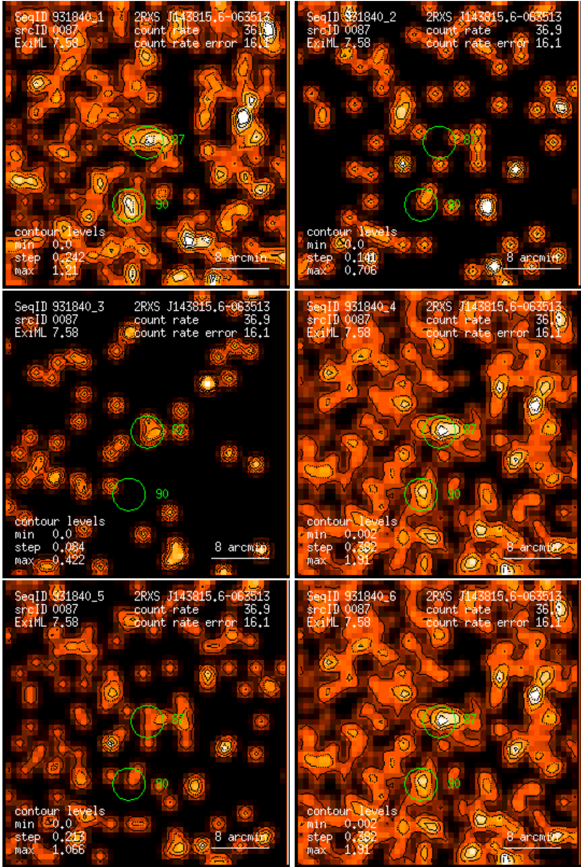
Figure 87: RASS 931840: detection 0087: band rate images, Gaussian filter: (1) PSPC channels 11 – 41, (2) 52 – 90, (3) 91 – 201, (4) 11 – 235, (5) 52 – 201, (6) 11 – 201. Broad band rates in counts/ks. Band rate contour levels in counts/ks/arcmin 2 .
