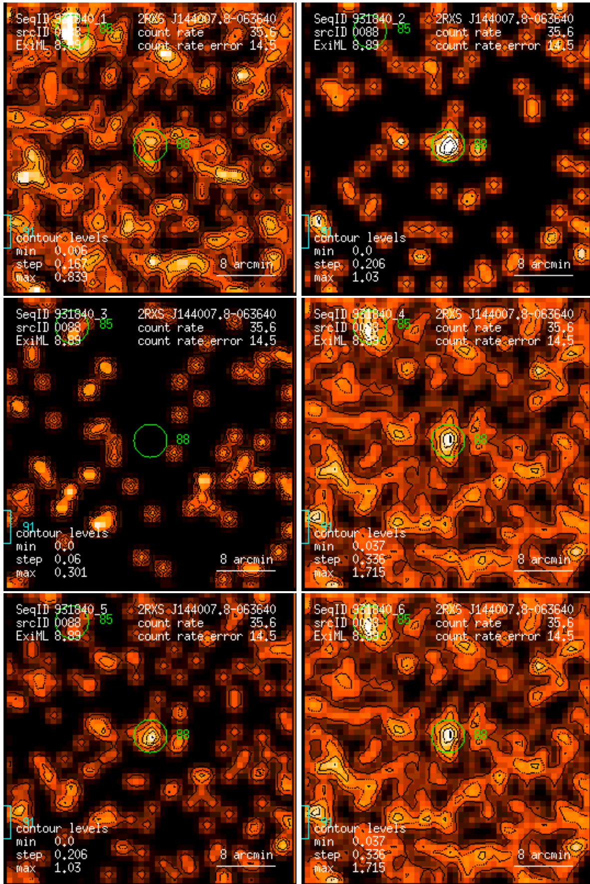
Figure 88: RASS 931840: detection 0088: band rate images, Gaussian filter: (1) PSPC channels 11 – 41, (2) 52 – 90, (3) 91 – 201, (4) 11 – 235, (5) 52 – 201, (6) 11 – 201. Broad band rates in counts/ks. Band rate contour levels in counts/ks/arcmin 2 .
