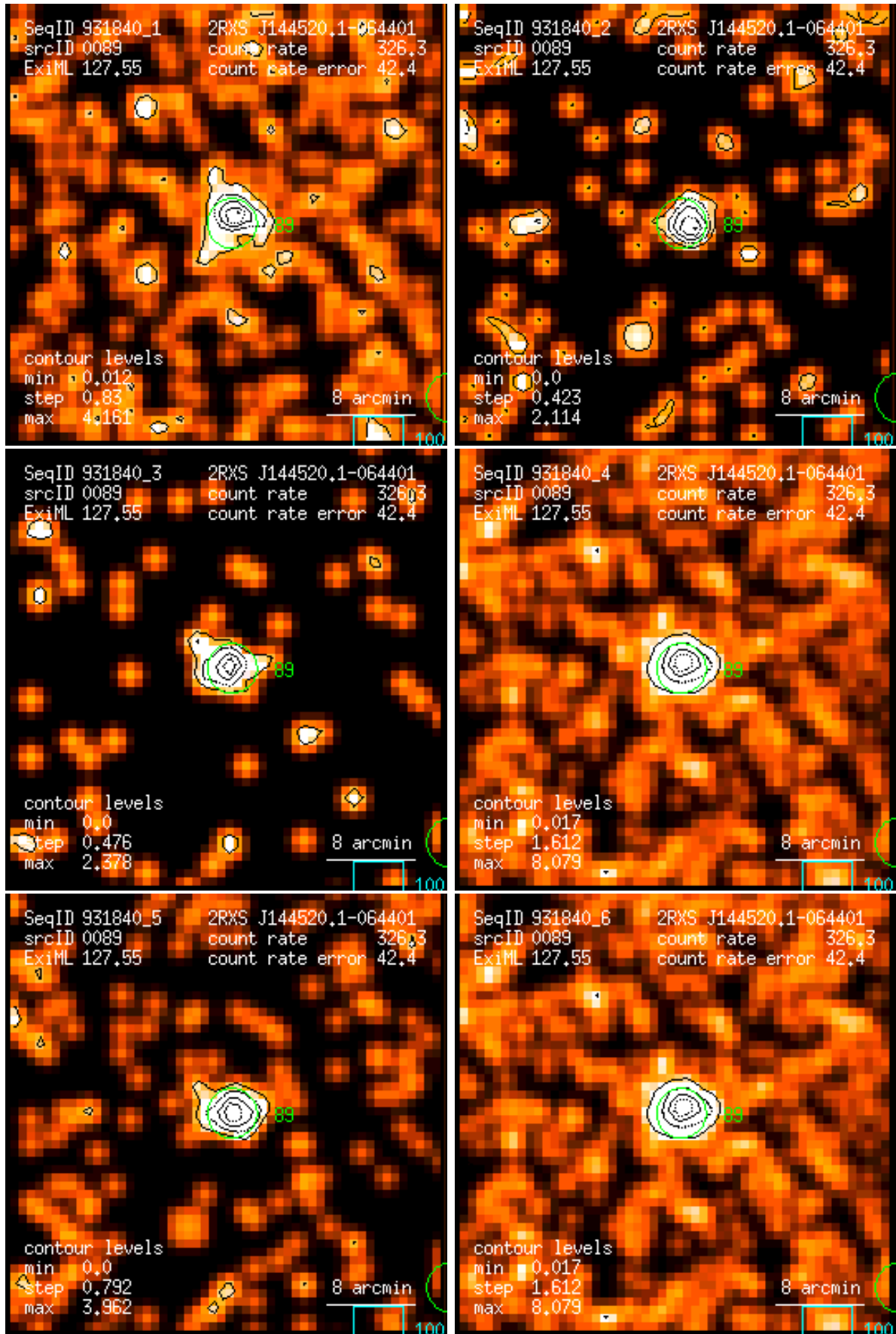
Figure 89: RASS 931840: detection 0089: band rate images, Gaussian filter: (1) PSPC channels 11 – 41, (2) 52 – 90, (3) 91 – 201, (4) 11 – 235, (5) 52 – 201, (6) 11 – 201. Broad band rates in counts/ks. Band rate contour levels in counts/ks/arcmin 2 .
