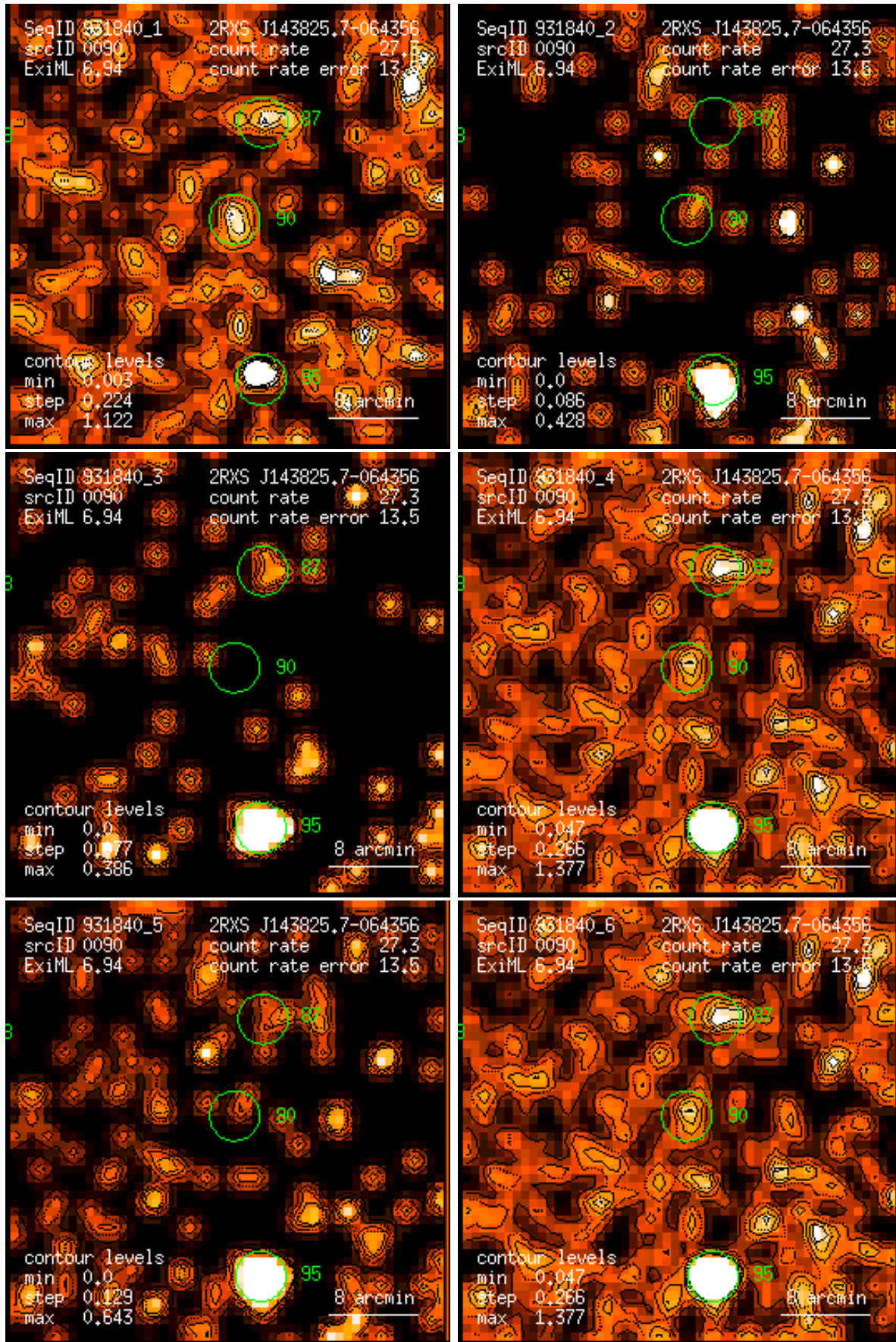
Figure 90: RASS 931840: detection 0090: band rate images, Gaussian filter: (1) PSPC channels 11 – 41, (2) 52 – 90, (3) 91 – 201, (4) 11 – 235, (5) 52 – 201, (6) 11 – 201. Broad band rates in counts/ks. Band rate contour levels in counts/ks/arcmin 2 .
