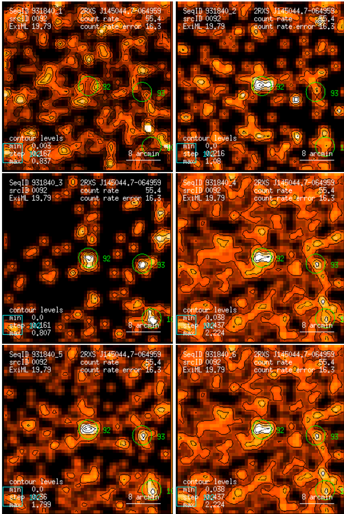
Figure 92: RASS 931840: detection 0092: band rate images, Gaussian filter: (1) PSPC channels 11 – 41, (2) 52 – 90, (3) 91 – 201, (4) 11 – 235, (5) 52 – 201, (6) 11 – 201. Broad band rates in counts/ks. Band rate contour levels in counts/ks/arcmin 2 .
