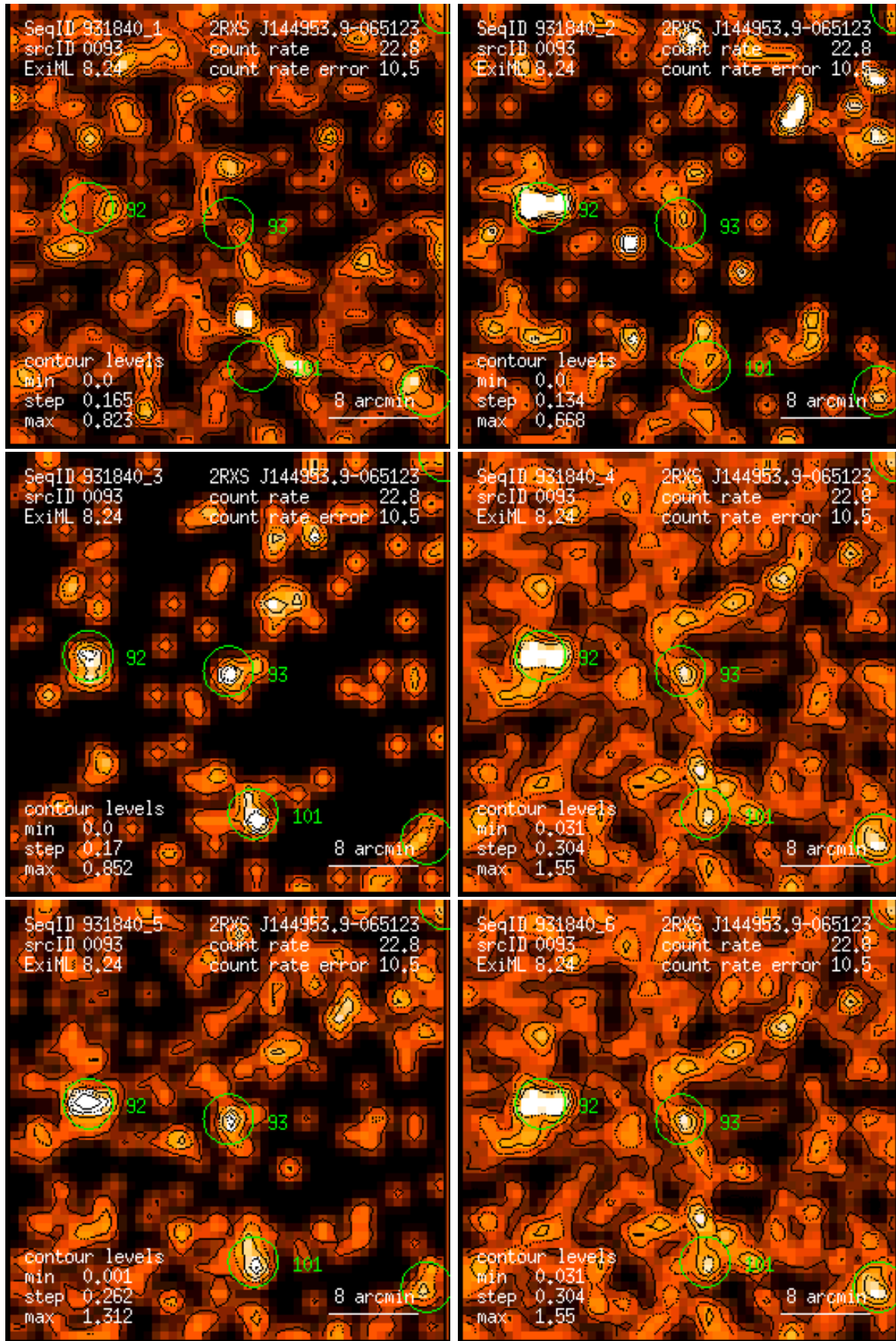
Figure 93: RASS 931840: detection 0093: band rate images, Gaussian filter: (1) PSPC channels 11 – 41, (2) 52 – 90, (3) 91 – 201, (4) 11 – 235, (5) 52 – 201, (6) 11 – 201. Broad band rates in counts/ks. Band rate contour levels in counts/ks/arcmin 2 .
