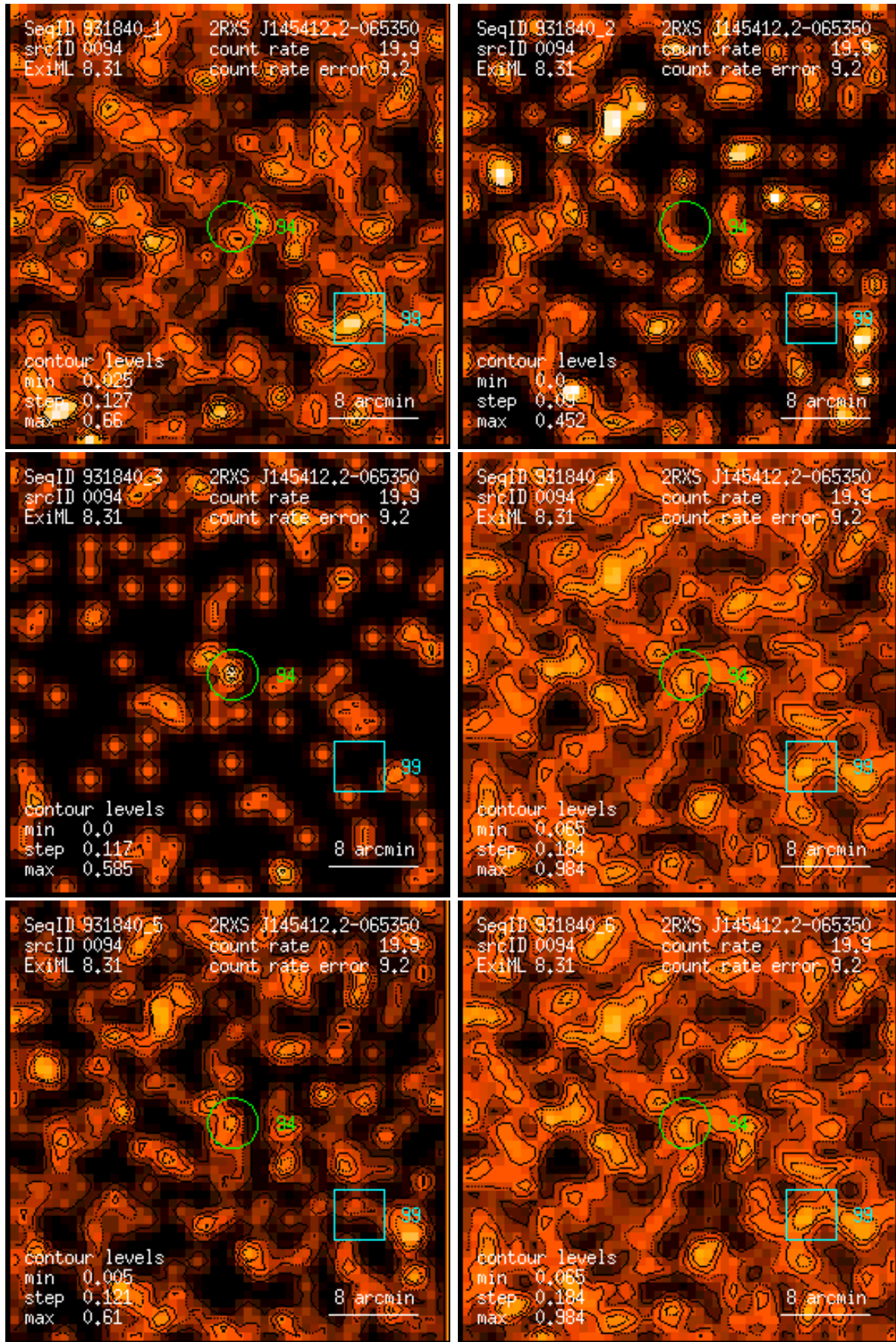
Figure 94: RASS 931840: detection 0094: band rate images, Gaussian filter: (1) PSPC channels 11 – 41, (2) 52 – 90, (3) 91 – 201, (4) 11 – 235, (5) 52 – 201, (6) 11 – 201. Broad band rates in counts/ks. Band rate contour levels in counts/ks/arcmin 2 .
