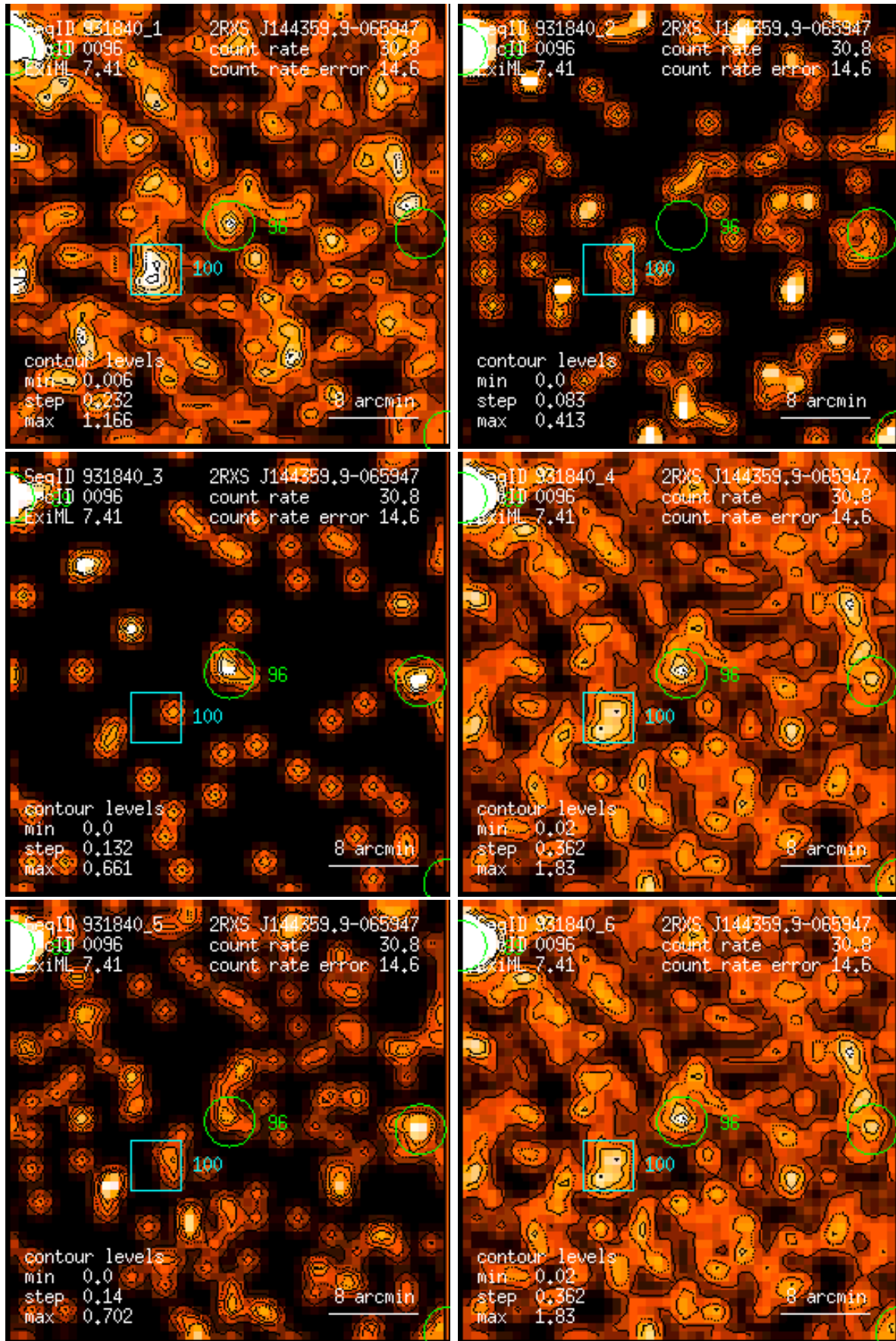
Figure 96: RASS 931840: detection 0096: band rate images, Gaussian filter: (1) PSPC channels 11 – 41, (2) 52 – 90, (3) 91 – 201, (4) 11 – 235, (5) 52 – 201, (6) 11 – 201. Broad band rates in counts/ks. Band rate contour levels in counts/ks/arcmin 2 .
