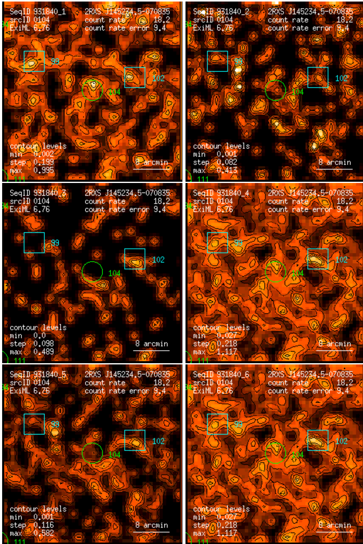
Figure 104: RASS 931840: detection 0104: band rate images, Gaussian filter: (1) PSPC channels 11 – 41, (2) 52 – 90, (3) 91 – 201, (4) 11 – 235, (5) 52 – 201, (6) 11 – 201. Broad band rates in counts/ks. Band rate contour levels in counts/ks/arcmin 2 .
