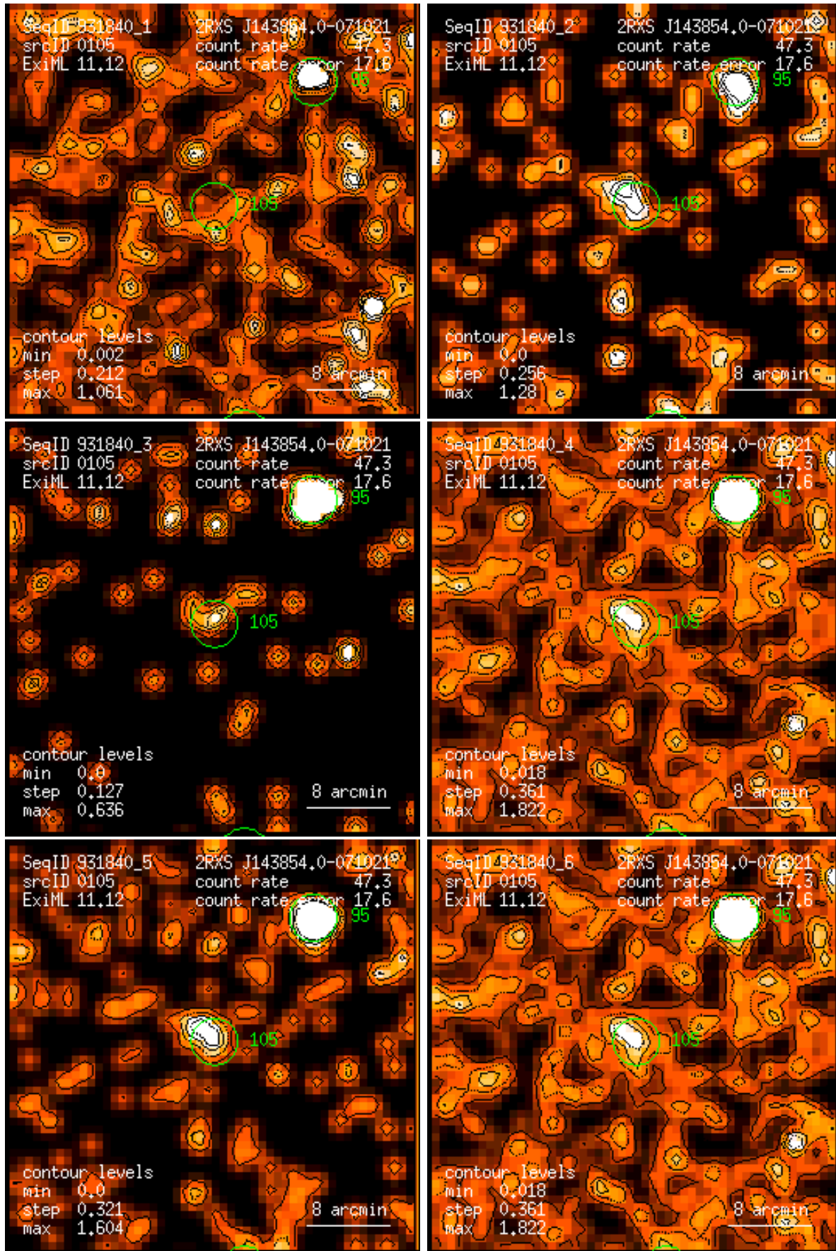
Figure 105: RASS 931840: detection 0105: band rate images, Gaussian filter: (1) PSPC channels 11 – 41, (2) 52 – 90, (3) 91 – 201, (4) 11 – 235, (5) 52 – 201, (6) 11 – 201. Broad band rates in counts/ks. Band rate contour levels in counts/ks/arcmin 2 .
