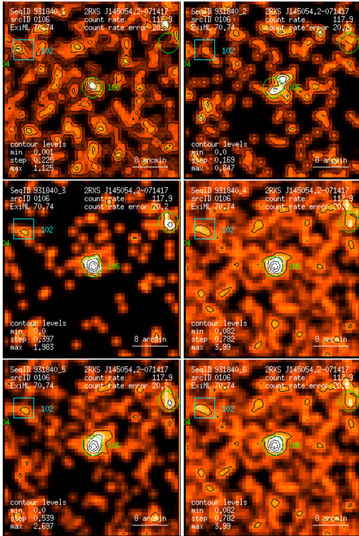
Figure 106: RASS 931840: detection 0106: band rate images, Gaussian filter: (1) PSPC channels 11 – 41, (2) 52 – 90, (3) 91 – 201, (4) 11 – 235, (5) 52 – 201, (6) 11 – 201. Broad band rates in counts/ks. Band rate contour levels in counts/ks/arcmin 2 .
