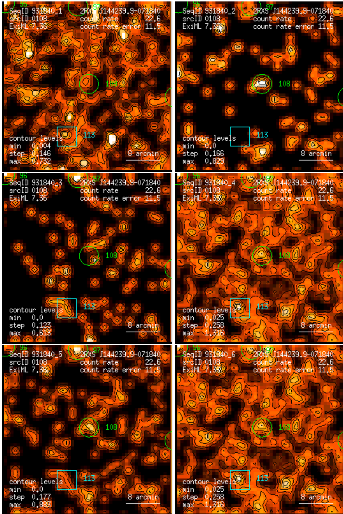
Figure 108: RASS 931840: detection 0108: band rate images, Gaussian filter: (1) PSPC channels 11 – 41, (2) 52 – 90, (3) 91 – 201, (4) 11 – 235, (5) 52 – 201, (6) 11 – 201. Broad band rates in counts/ks. Band rate contour levels in counts/ks/arcmin 2 .
