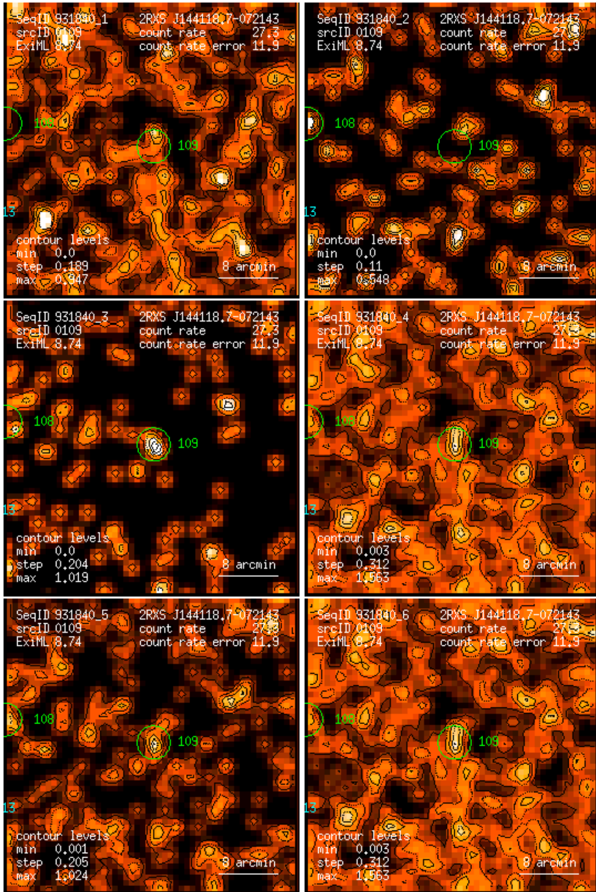
Figure 109: RASS 931840: detection 0109: band rate images, Gaussian filter: (1) PSPC channels 11 – 41, (2) 52 – 90, (3) 91 – 201, (4) 11 – 235, (5) 52 – 201, (6) 11 – 201. Broad band rates in counts/ks. Band rate contour levels in counts/ks/arcmin 2 .
