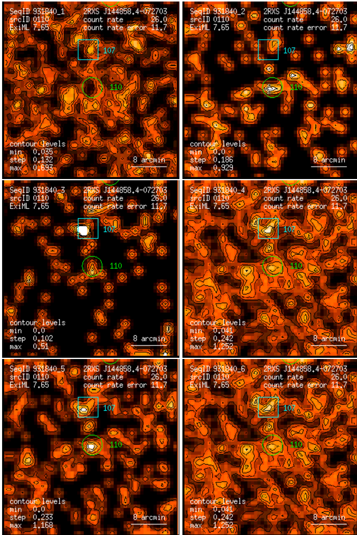
Figure 110: RASS 931840: detection 0110: band rate images, Gaussian filter: (1) PSPC channels 11 – 41, (2) 52 – 90, (3) 91 – 201, (4) 11 – 235, (5) 52 – 201, (6) 11 – 201. Broad band rates in counts/ks. Band rate contour levels in counts/ks/arcmin 2 .
