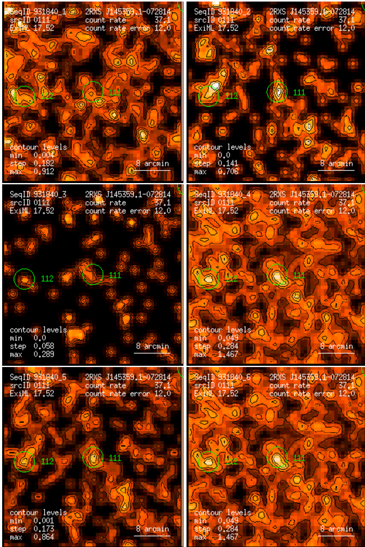
Figure 111: RASS 931840: detection 0111: band rate images, Gaussian filter: (1) PSPC channels 11 – 41, (2) 52 – 90, (3) 91 – 201, (4) 11 – 235, (5) 52 – 201, (6) 11 – 201. Broad band rates in counts/ks. Band rate contour levels in counts/ks/arcmin 2 .
