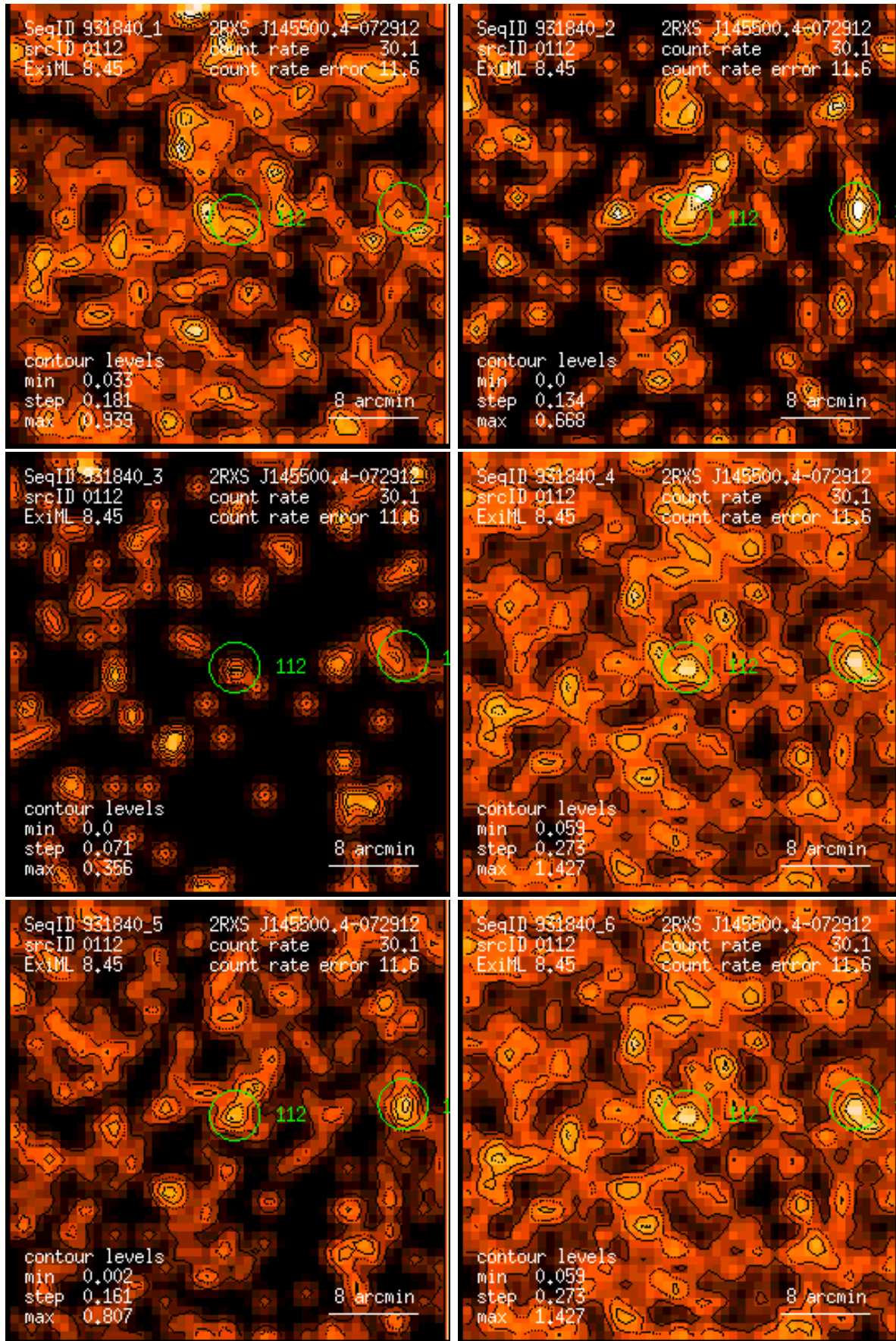
Figure 112: RASS 931840: detection 0112: band rate images, Gaussian filter: (1) PSPC channels 11 – 41, (2) 52 – 90, (3) 91 – 201, (4) 11 – 235, (5) 52 – 201, (6) 11 – 201. Broad band rates in counts/ks. Band rate contour levels in counts/ks/arcmin 2 .
