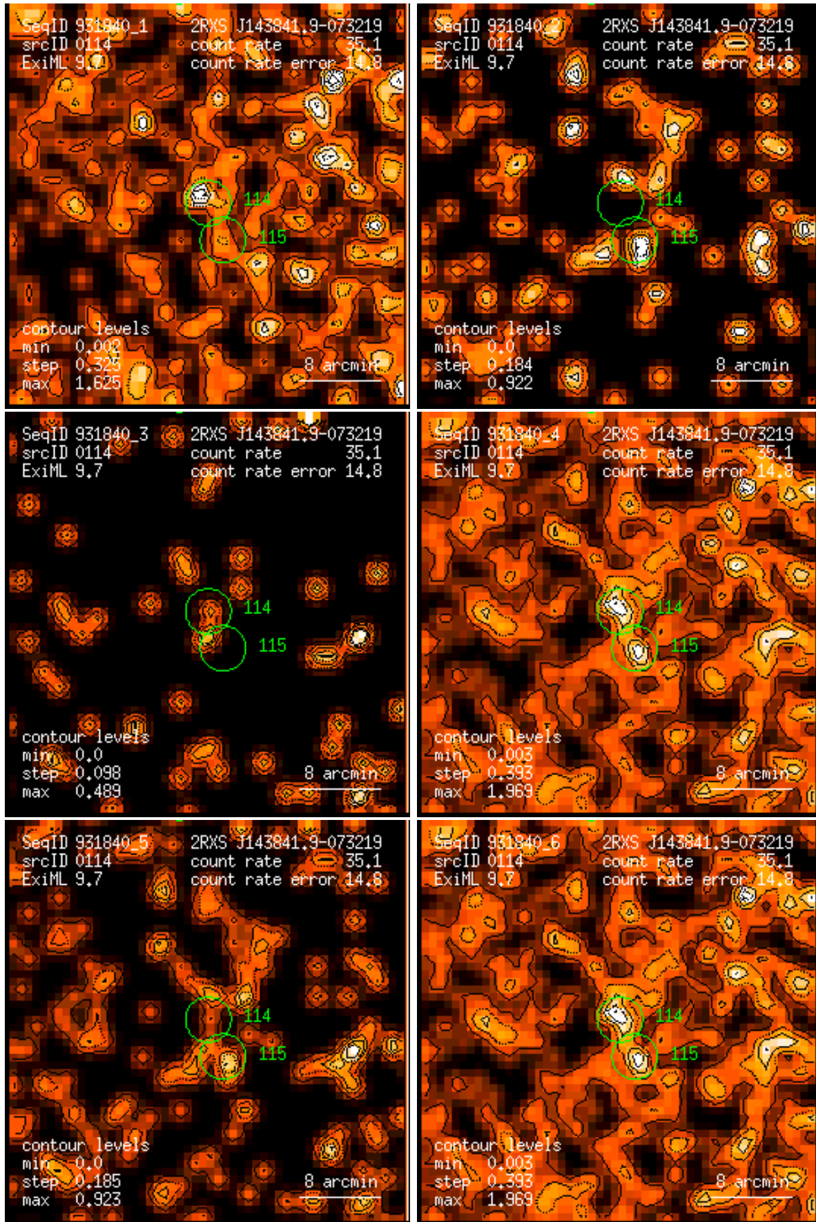
Figure 114: RASS 931840: detection 0114: band rate images, Gaussian filter: (1) PSPPC channels 11 – 41, (2) 52 – 90, (3) 91 – 201, (4) 11 – 235, (5) 52 – 201, (6) 11 – 201. Broad band rates in counts/ks. Band rate contour levels in counts/ks/arcmin 2 .
