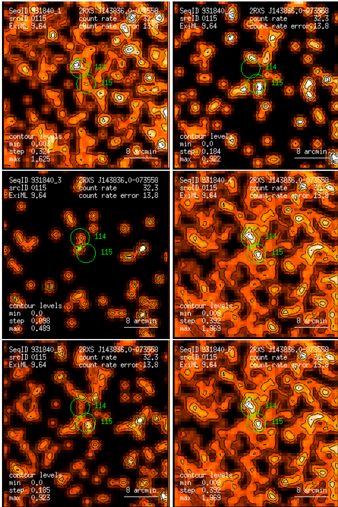
Figure 115: RASS 931840: detection 0115: band rate images, Gaussian filter: (1) PSPC channels 11 – 41, (2) 52 – 90, (3) 91 – 201, (4) 11 – 235, (5) 52 – 201, (6) 11 – 201. Broad band rates in counts/ks. Band rate contour levels in counts/ks/arcmin 2 .
