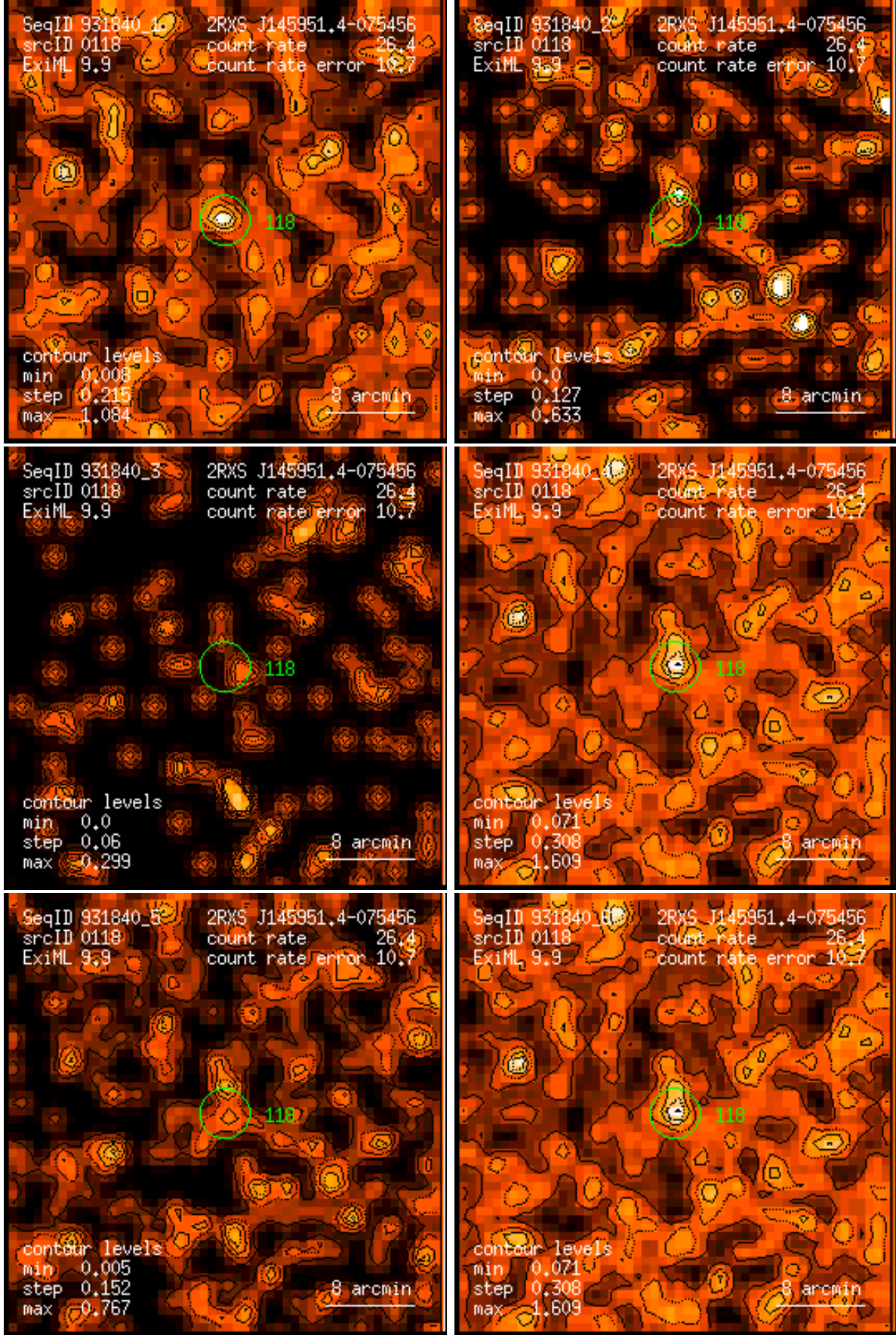
Figure 118: RASS 931840: detection 0118: band rate images, Gaussian filter: (1) PSPC channels 11 – 41, (2) 52 – 90, (3) 91 – 201, (4) 11 – 235, (5) 52 – 201, (6) 11 – 201. Broad band rates in counts/ks. Band rate contour levels in counts/ks/arcmin 2 .
