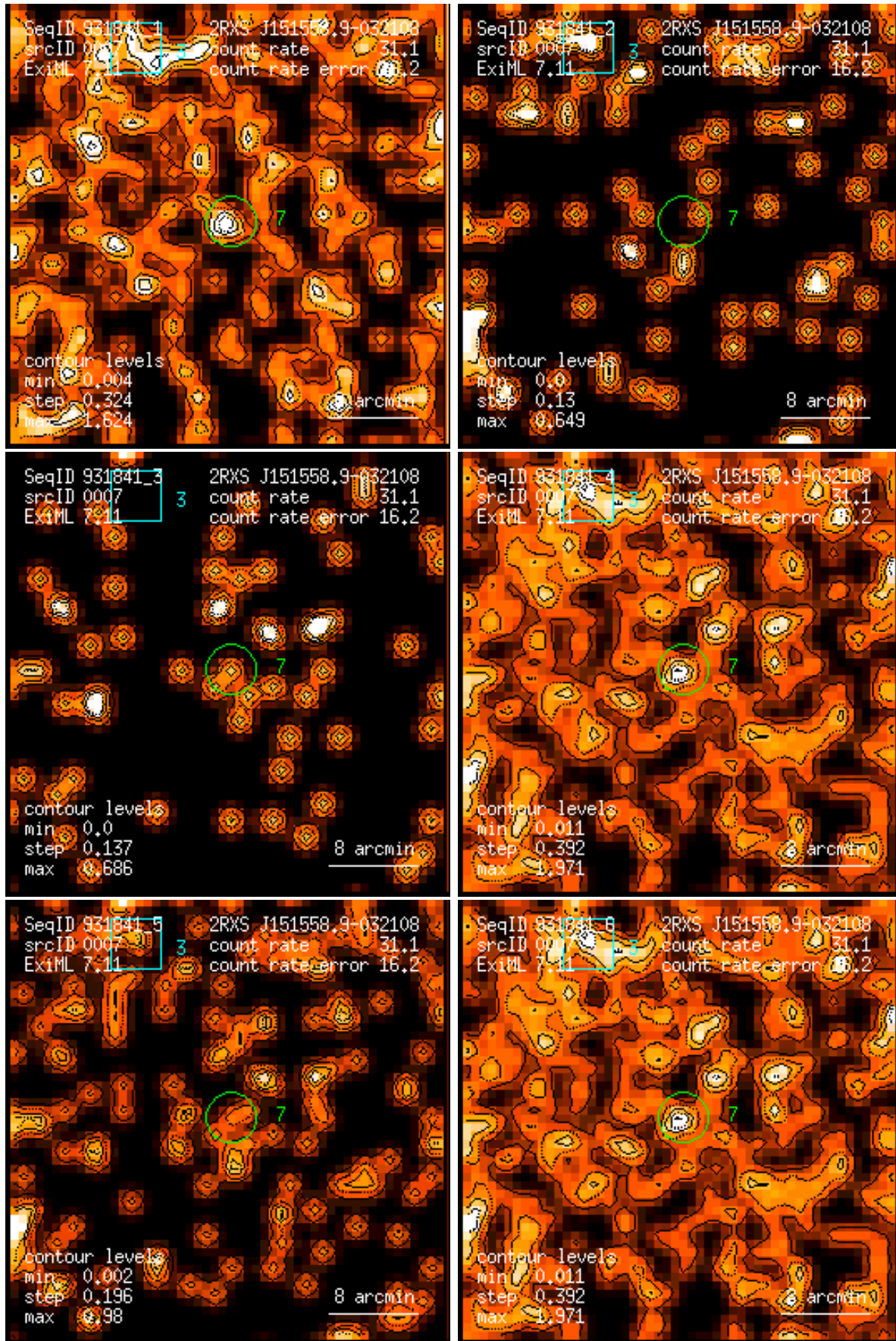
Figure 7: RASS 931841: detection 0007: band rate images, Gaussian filter: (1) PSPC channels 11 – 41, (2) 52 – 90, (3) 91 – 201, (4) 11 – 235, (5) 52 – 201, (6) 11 – 201. Broad band rates in counts/ks. Band rate contour levels in counts/ks/arcmin 2 .
