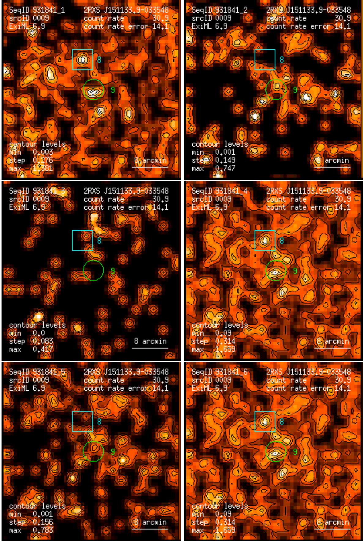
Figure 9: RASS 931841: detection 0009: band rate images, Gaussian filter: (1) PSPC channels 11 – 41, (2) 52 – 90, (3) 91 – 201, (4) 11 – 235, (5) 52 – 201, (6) 11 – 201. Broad band rates in counts/ks. Band rate contour levels in counts/ks/arcmin 2 .
