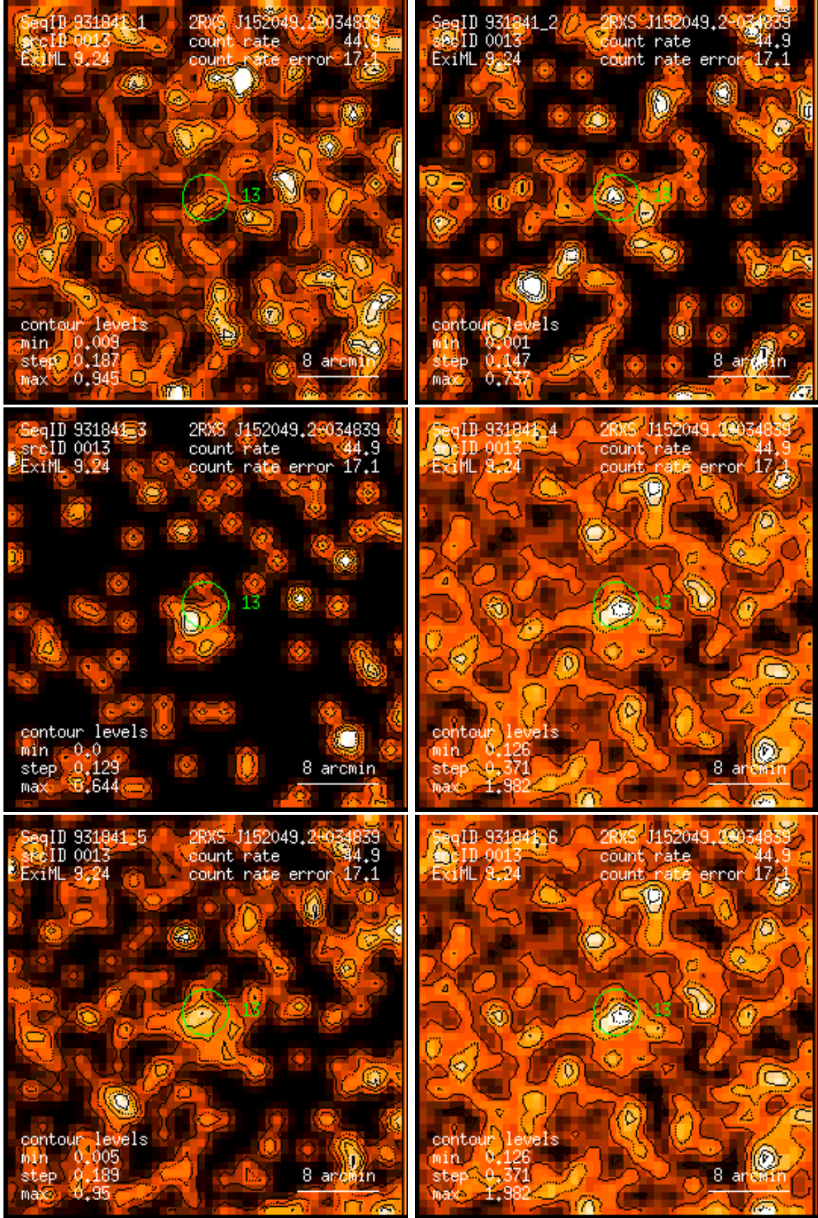
Figure 13: RASS 931841: detection 0013: band rate images, Gaussian filter: (1) PSPC channels 11 – 41, (2) 52 – 90, (3) 91 – 201, (4) 11 – 235, (5) 52 – 201, (6) 11 – 201. Broad band rates in counts/ks. Band rate contour levels in counts/ks/arcmin 2 .
