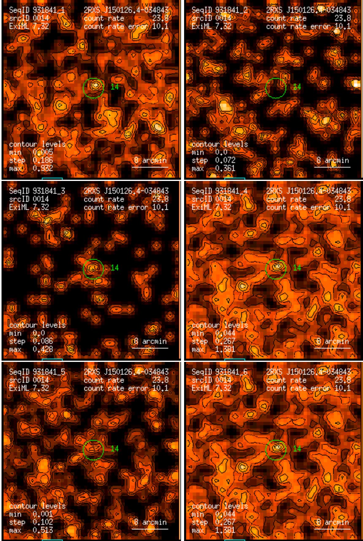
Figure 14: RASS 931841: detection 0014: band rate images, Gaussian filter: (1) PSPC channels 11 – 41, (2) 52 – 90, (3) 91 – 201, (4) 11 – 235, (5) 52 – 201, (6) 11 – 201. Broad band rates in counts/ks. Band rate contour levels in counts/ks/arcmin 2 .
